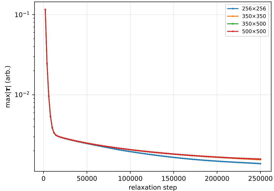
(b) residual torque (edge-limited)
