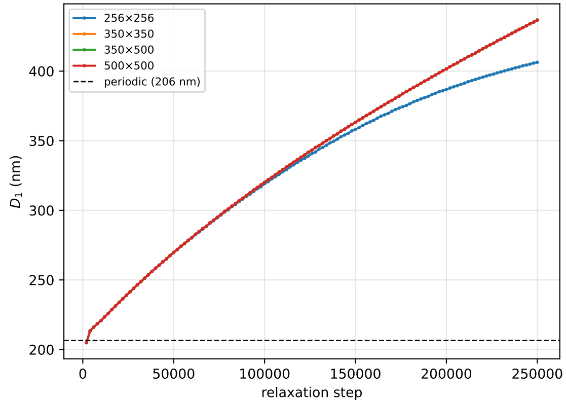
(a) diameter: monotonic expansion
