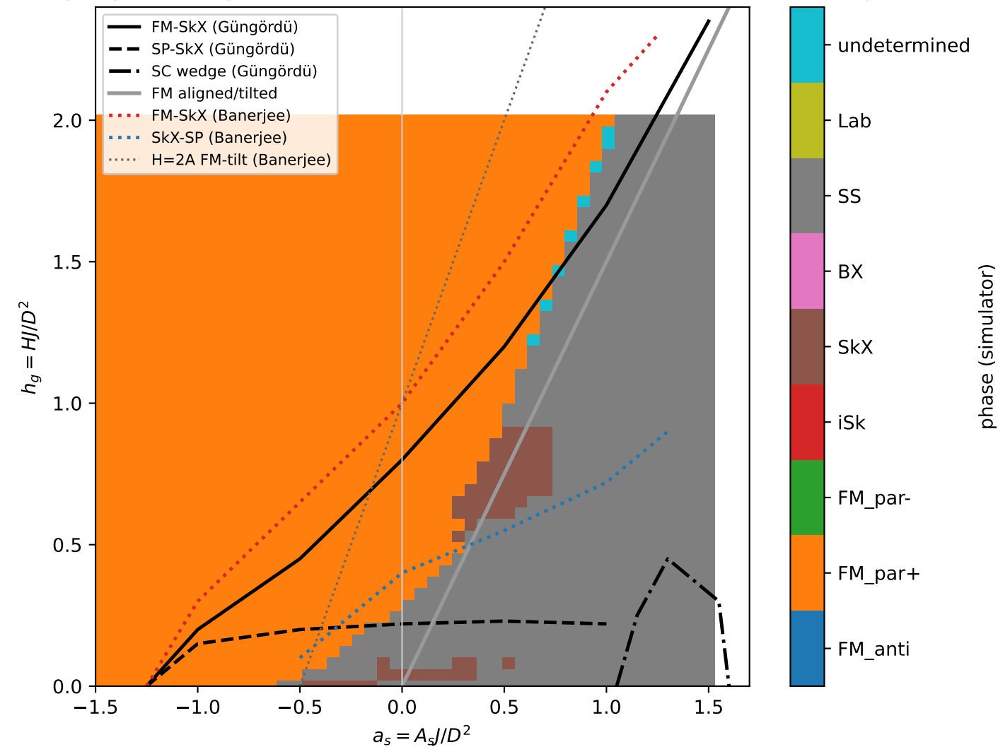
rdü Fig. 3 phase diagram ( D = 1.50 \text{ mJ/m}^2 , 50 \times 50 cells, 64 \times 64 lattice, demag off)
