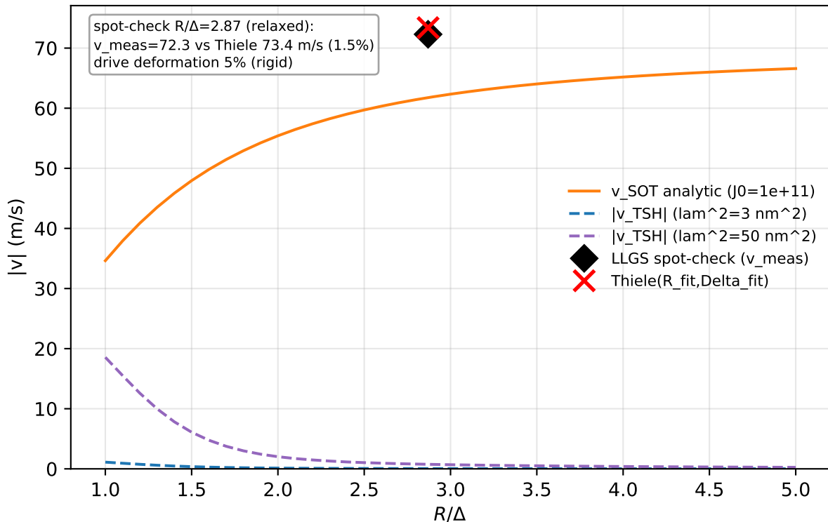
Pham 2024 Fig. S49 Thiele speeds (Set B, D=0.62 \text{ mJ/m}^2 )
