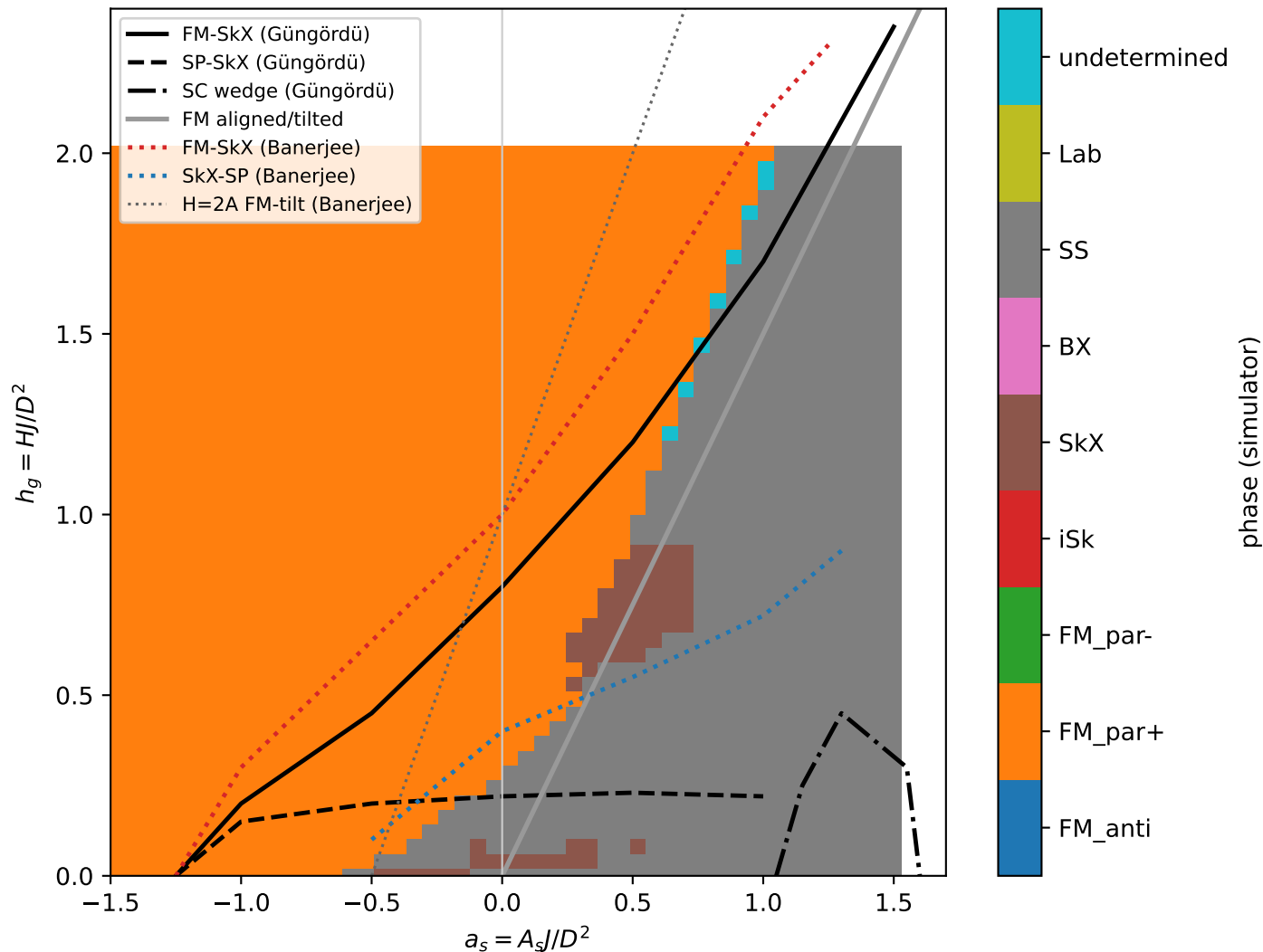
rdü Fig. 3 phase diagram ( D = 1.50 \text{ mJ/m}^2 , 50x50 cells, 64x64 lattice, demag off)
