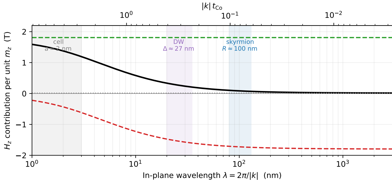
PMA vs slab demag: per-mode spectrum ( K_{\text{top}}=1.294 \text{ MJ/m}^3 , \mu_0 M_s=1.80 \text{ T} )
