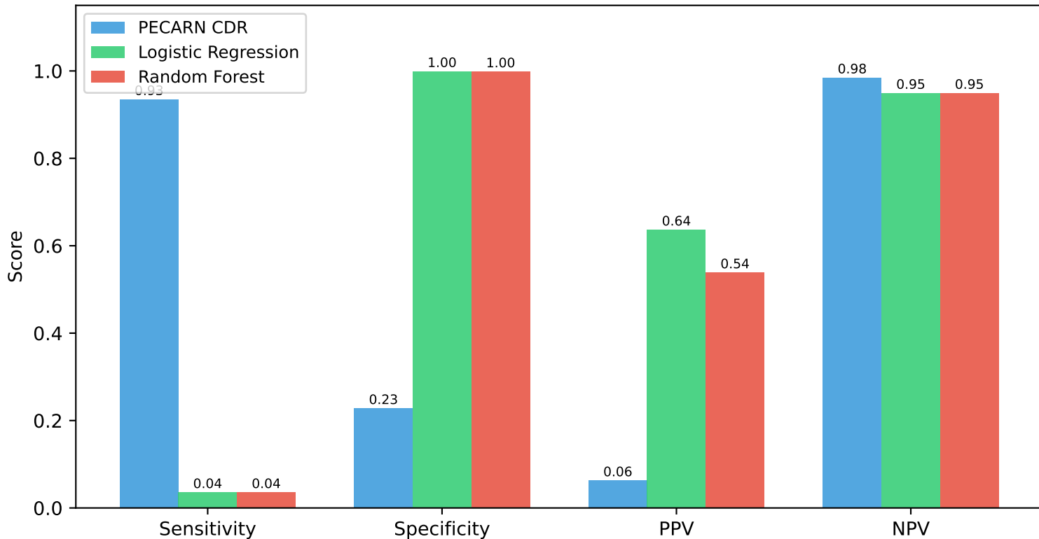
Diagnostic performance: Sensitivity, Specificity, PPV, NPV
