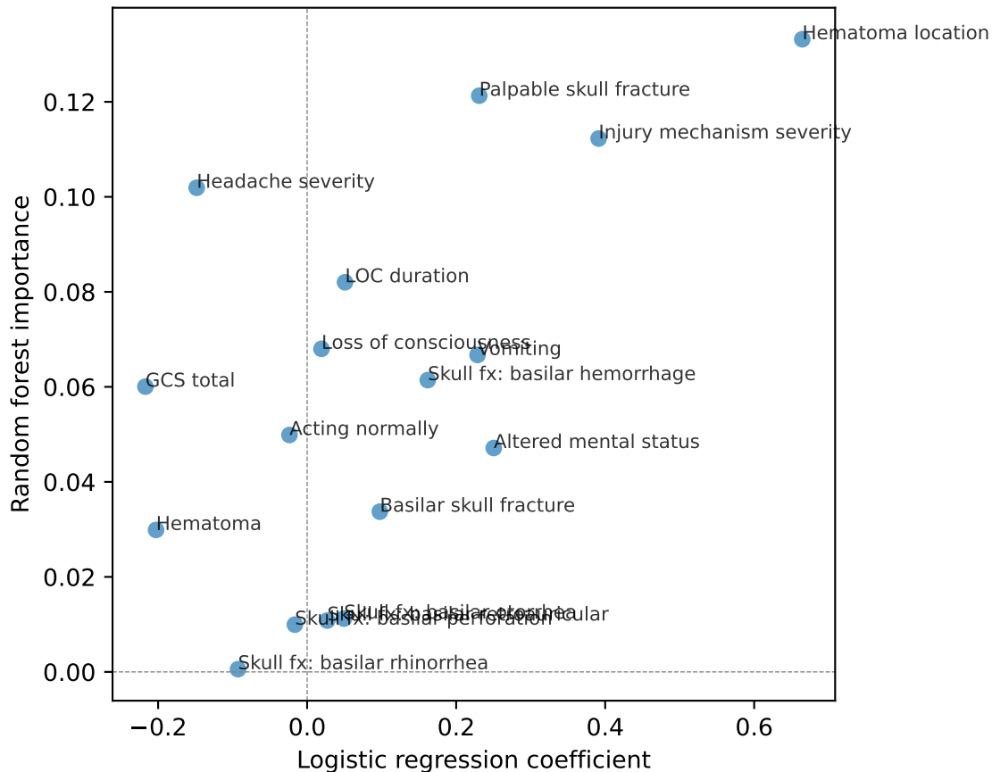
Model alignment: LR vs RF predictor emphasis
