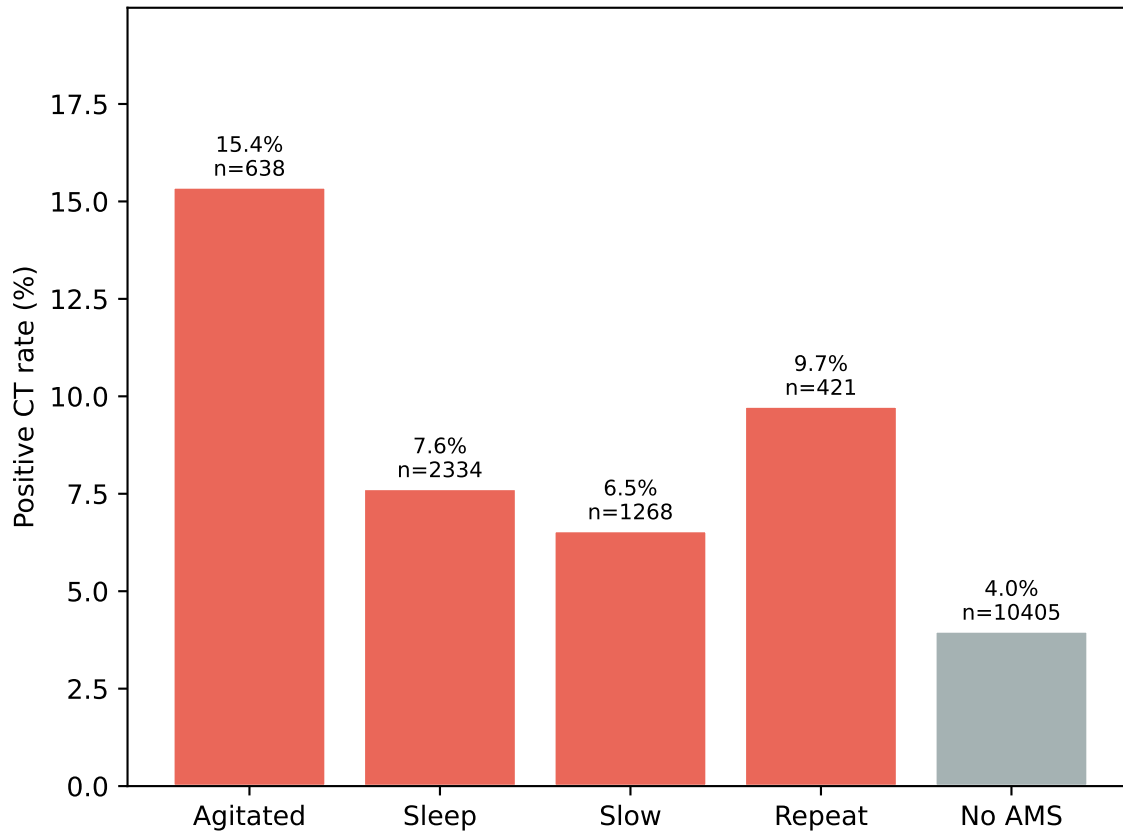
PosCT Rate by AMS Subtype
