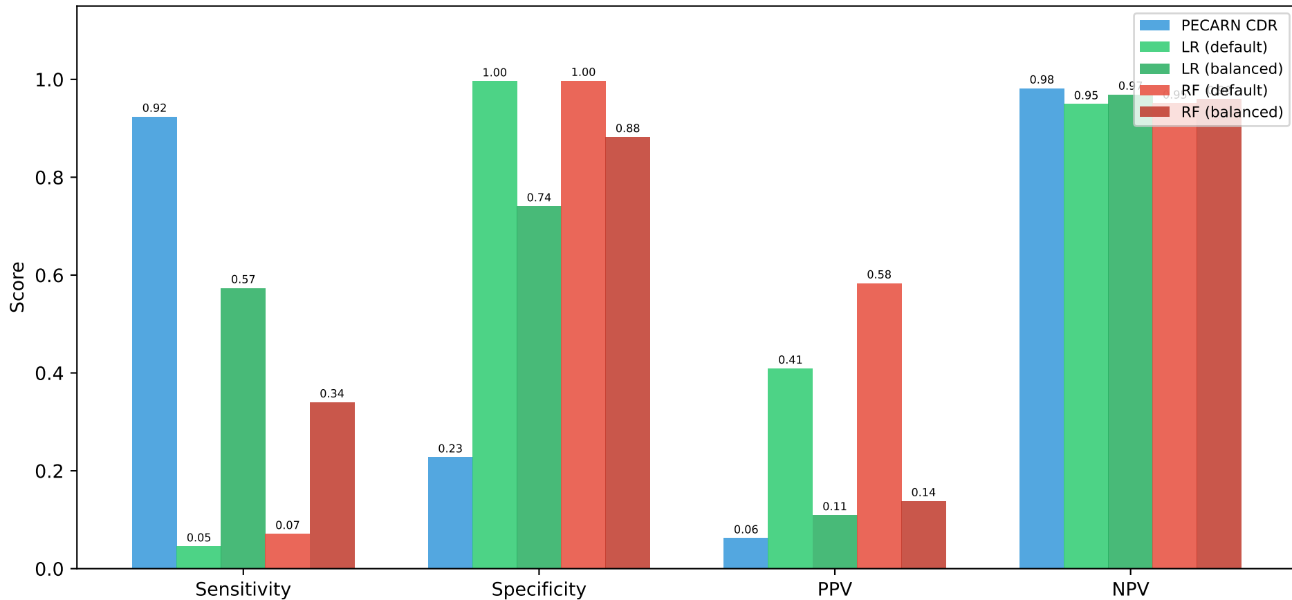
Diagnostic Performance: Default vs Class-Weighted Models
