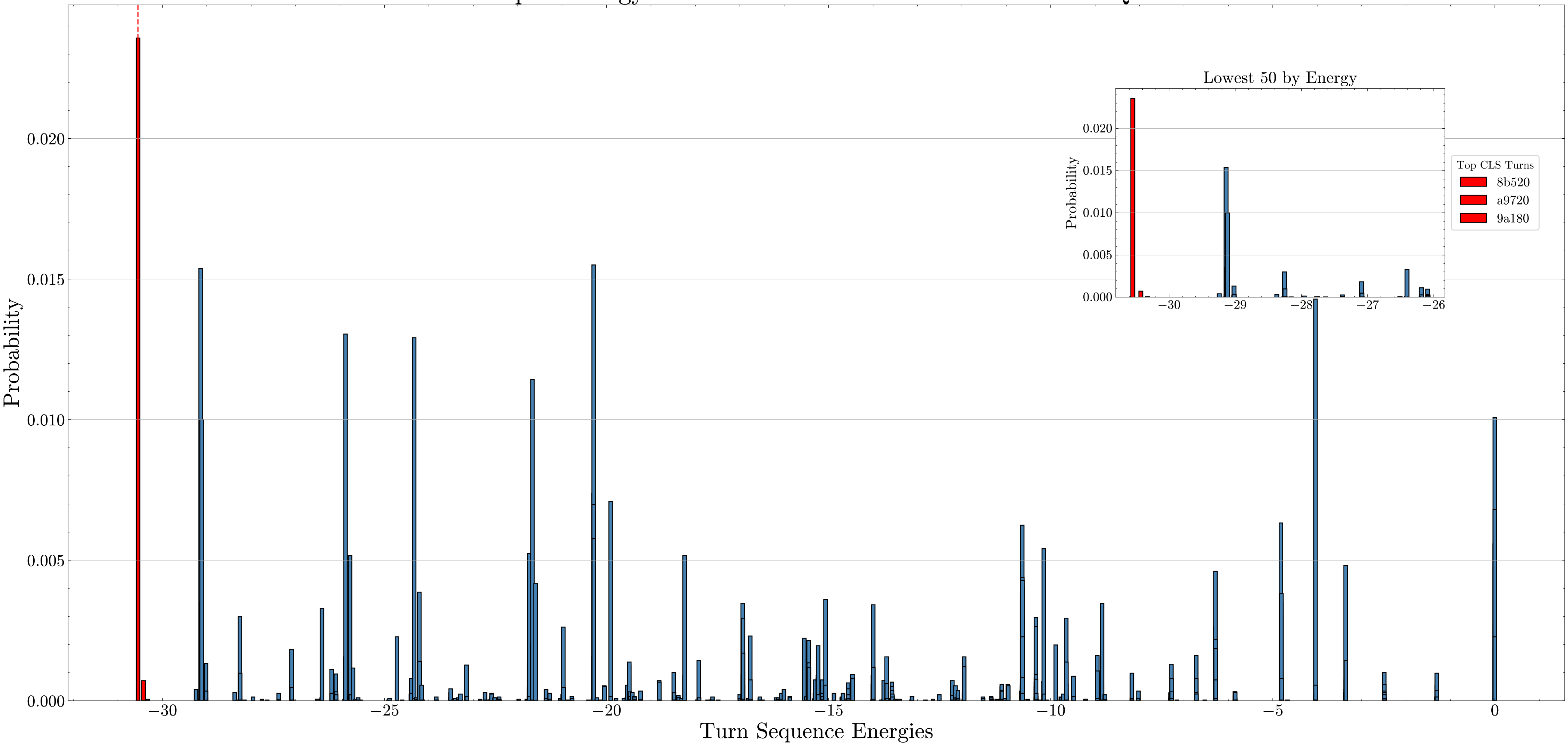
Sampled energy distribution from ibm "cleveland with VQEC
