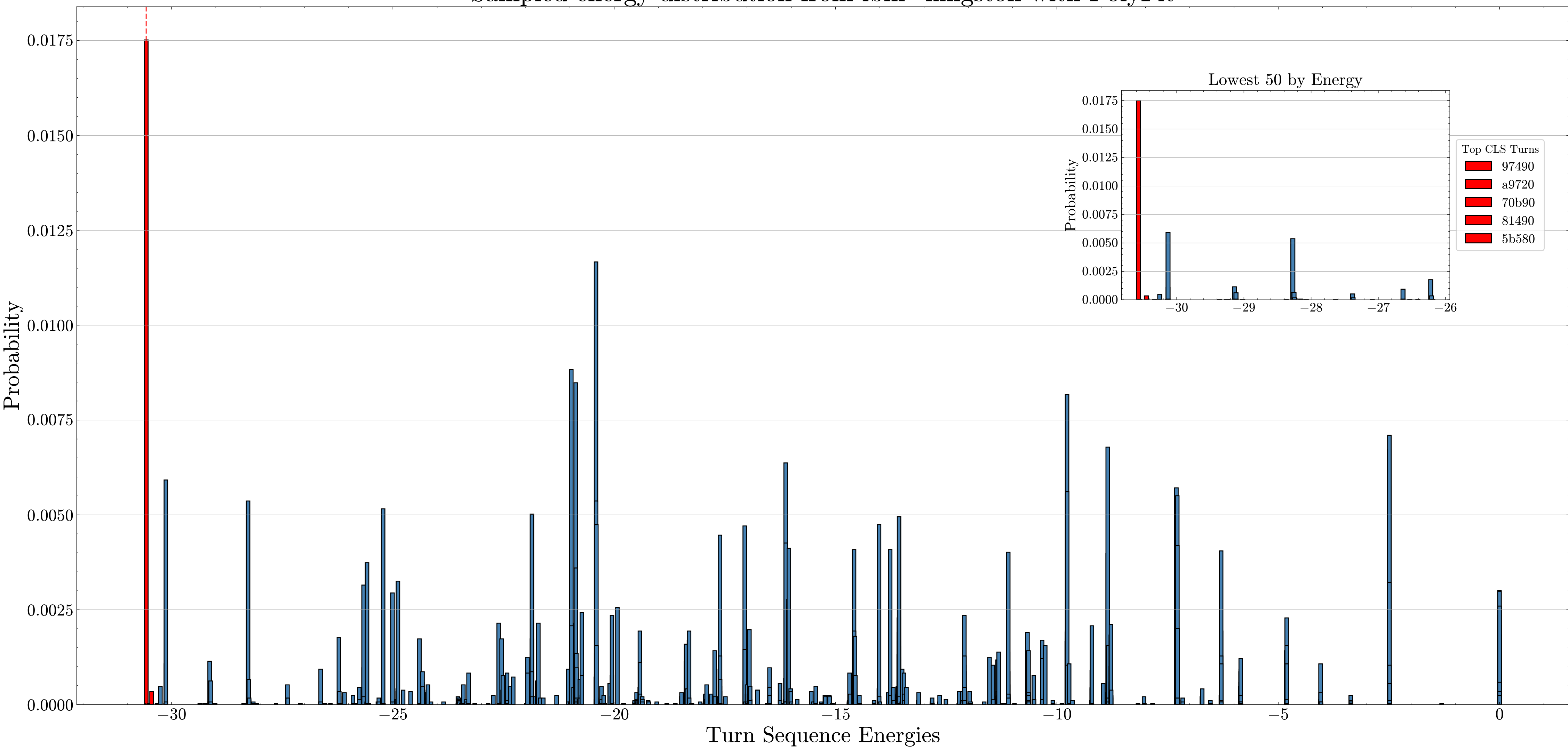
Sampled energy distribution from ibm“kingston with PolyFit
