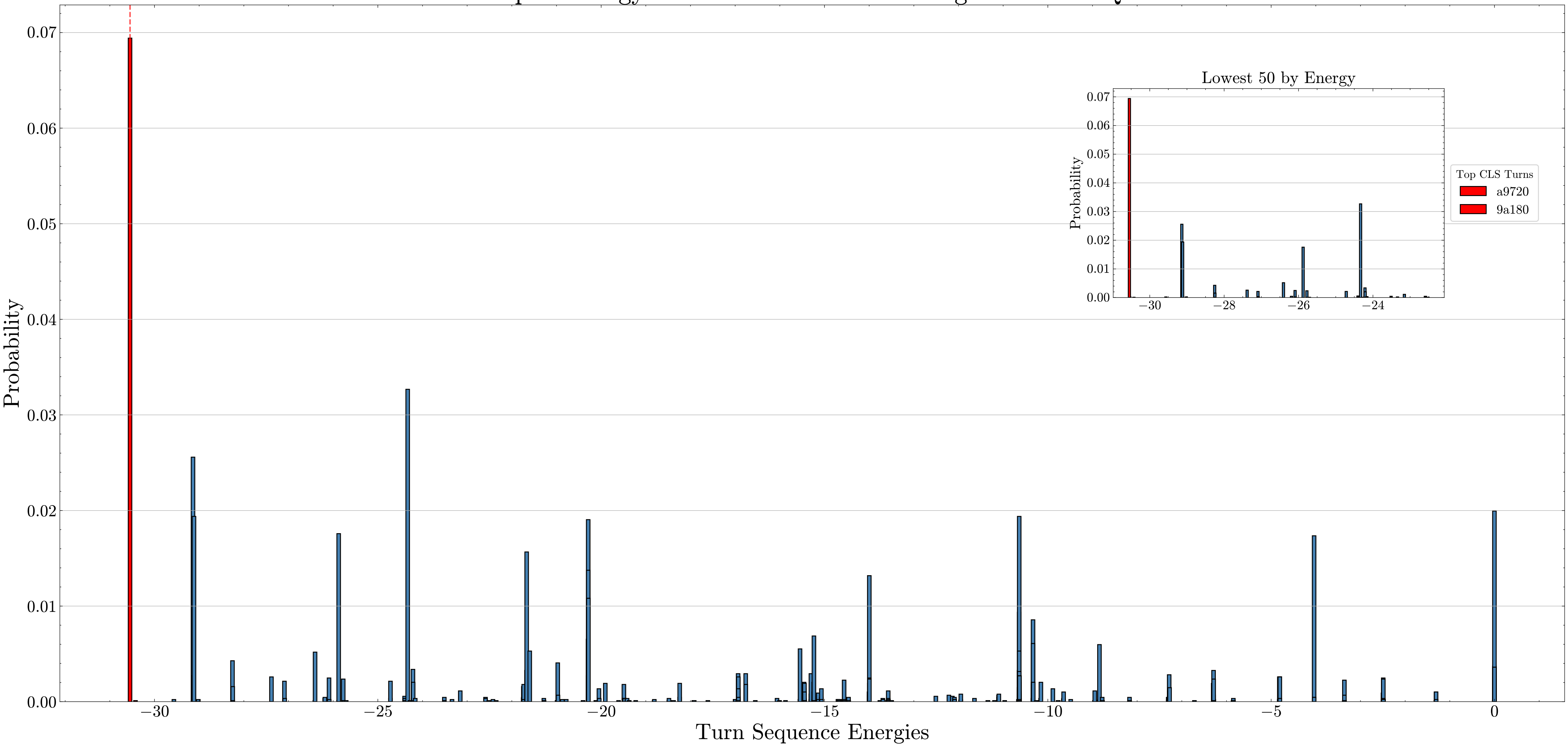
Sampled energy distribution from ibm“kingston with VQEC
