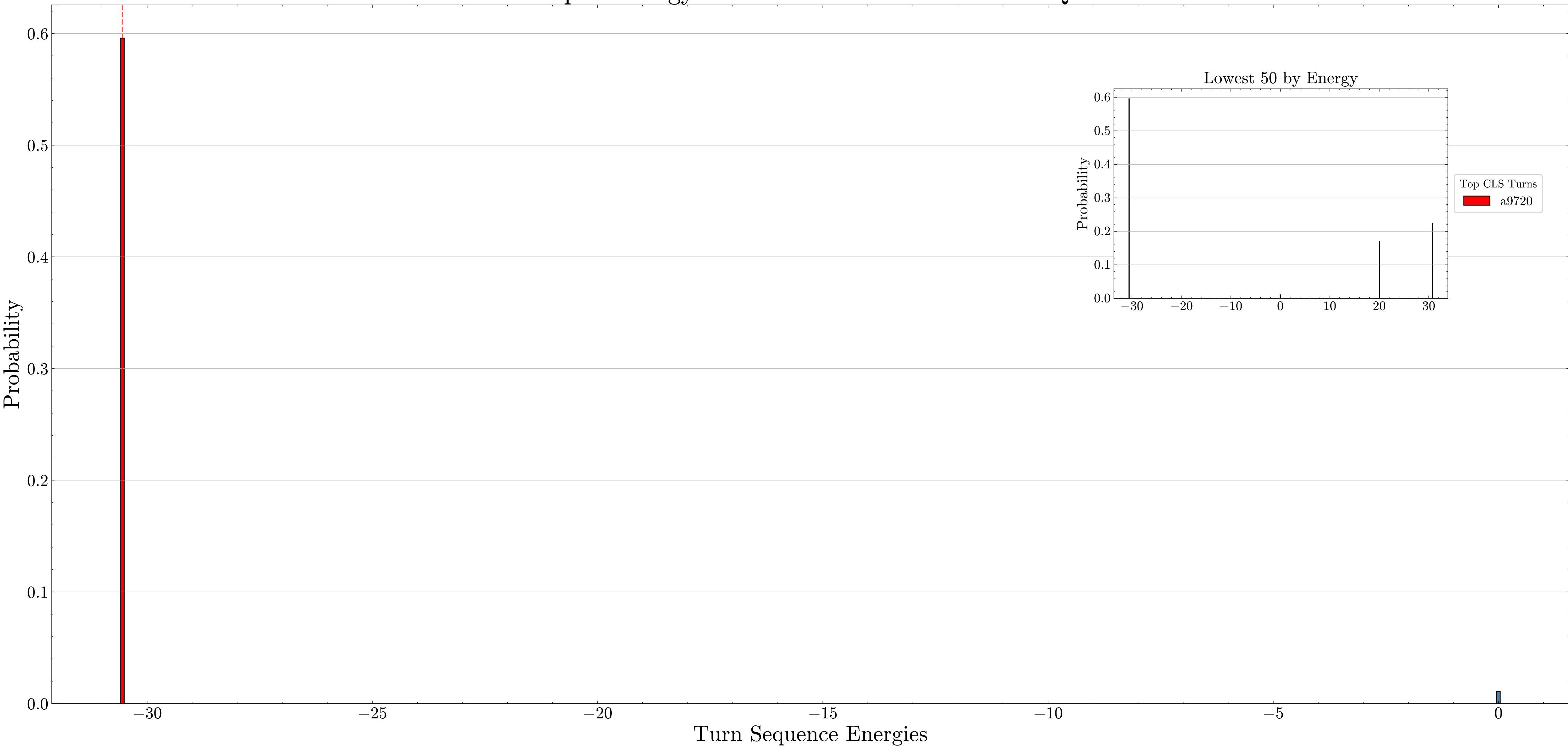
Sampled energy distribution from MPS with VQEC
