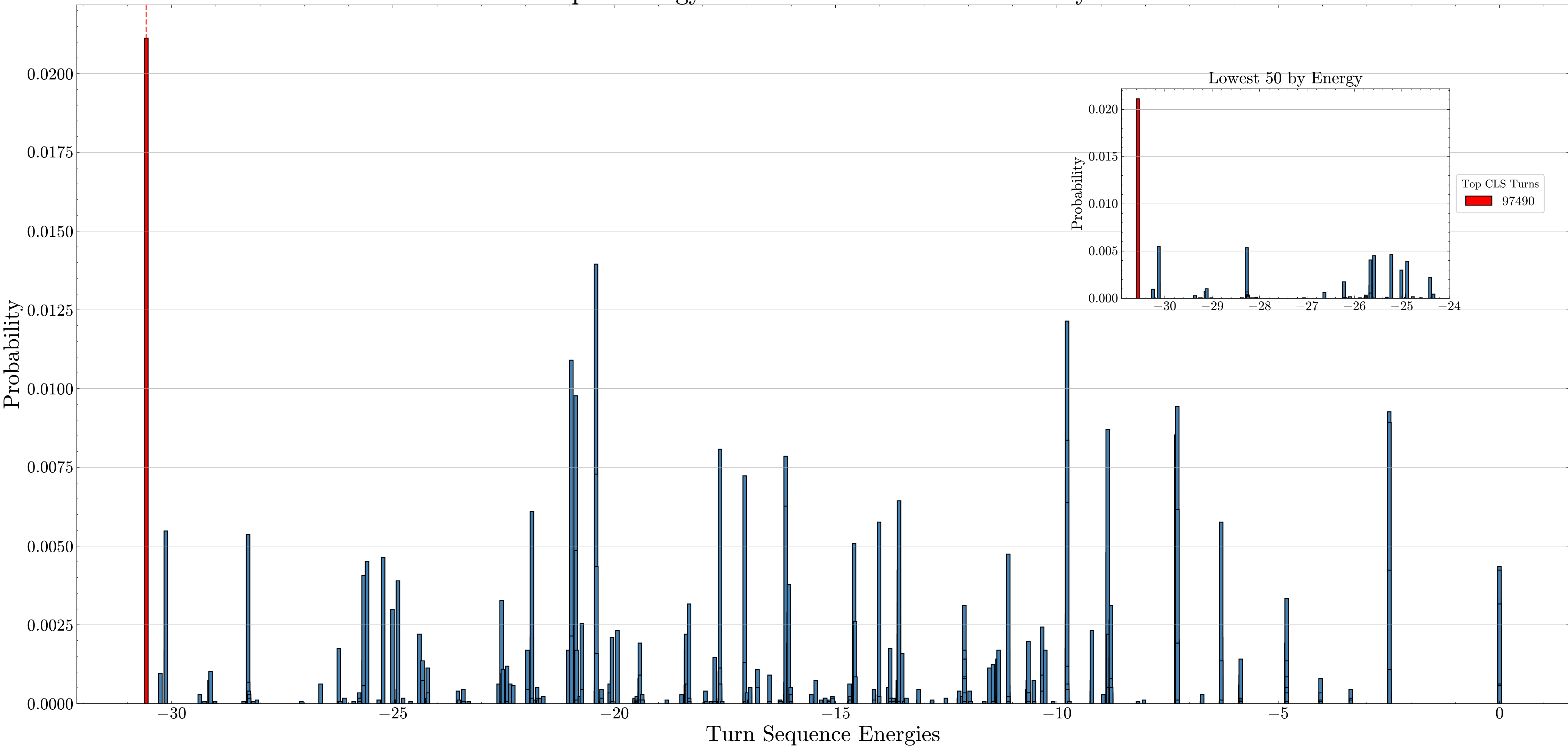
Sampled energy distribution from MPS with PolyFit
