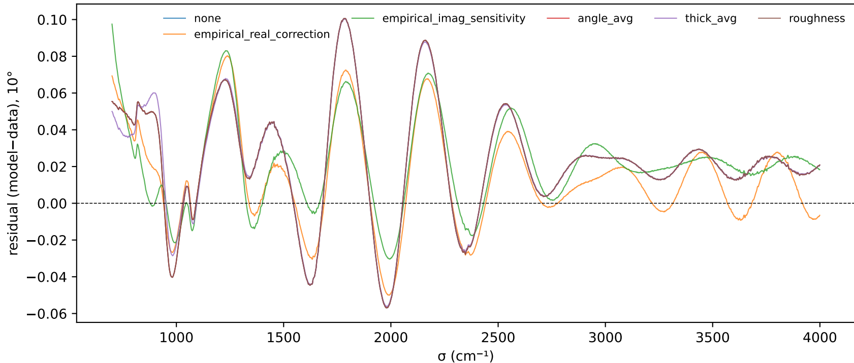
Study C: Si residual morphology by high-frequency mechanism
