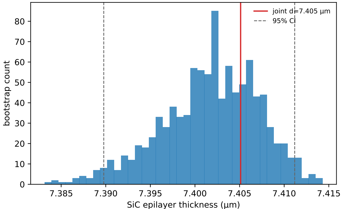
SiC joint-fit thickness: wild bootstrap (seed 20260601, n=1000)
