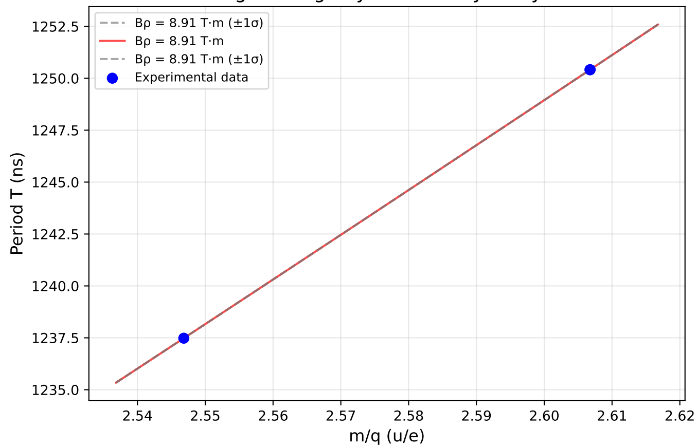
Magnetic rigidity uncertainty analysis
