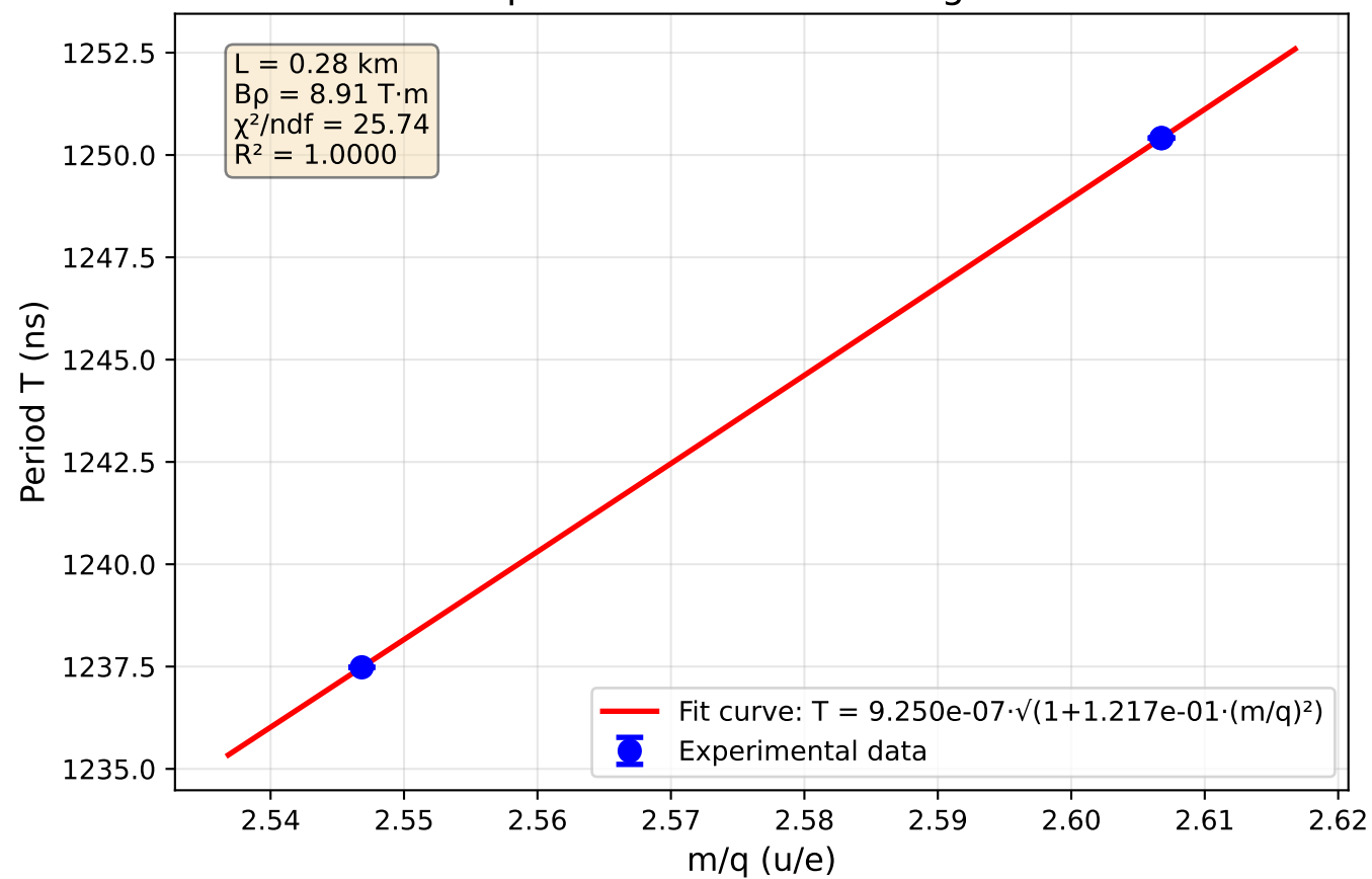
Ion period vs mass-to-charge ratio
