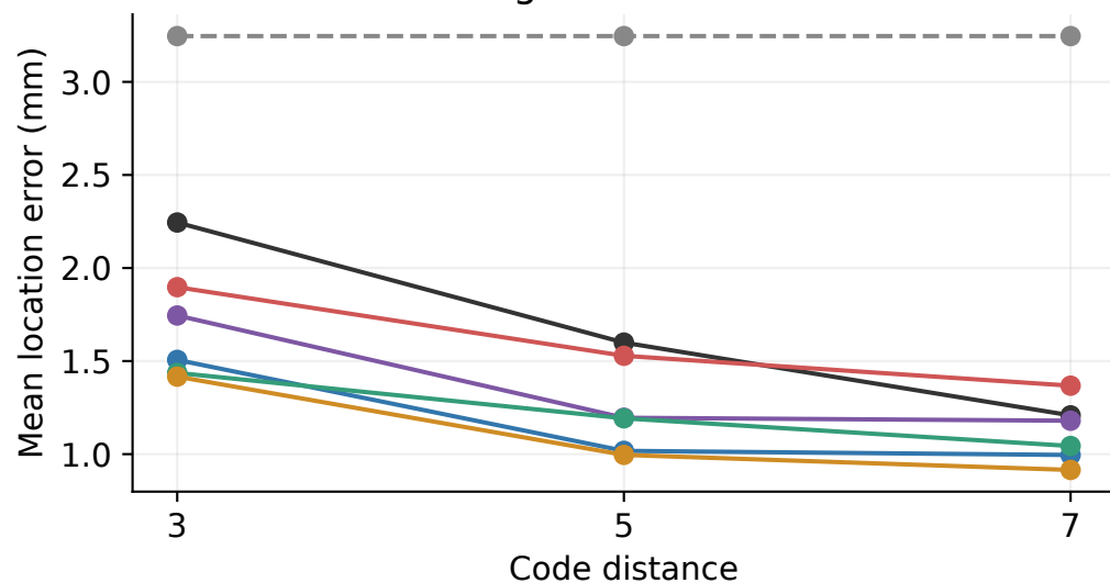
Strong circular events
