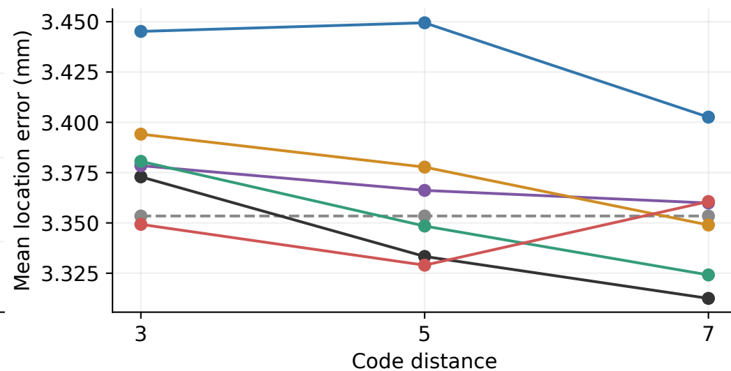
Strong elliptical events
