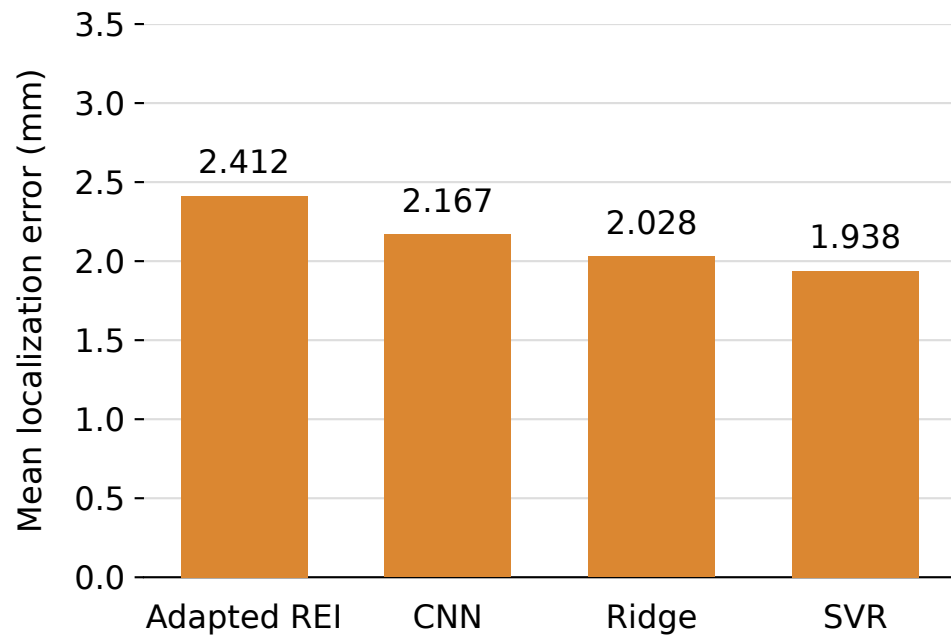
Strong elliptical events
