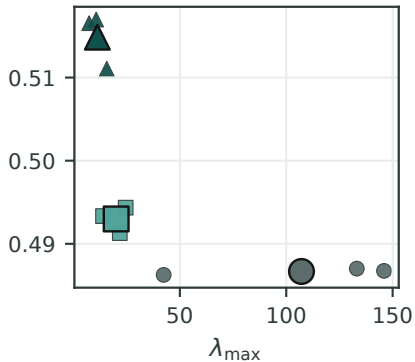
(b) CIFAR-100-C ResNet-18
