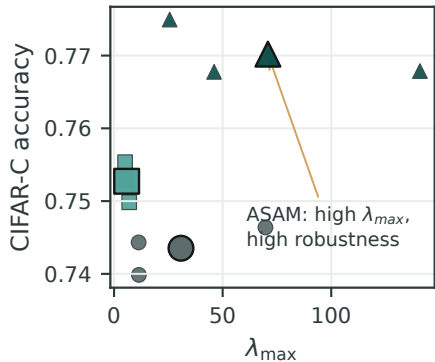
(a) CIFAR-10-C ResNet-18
