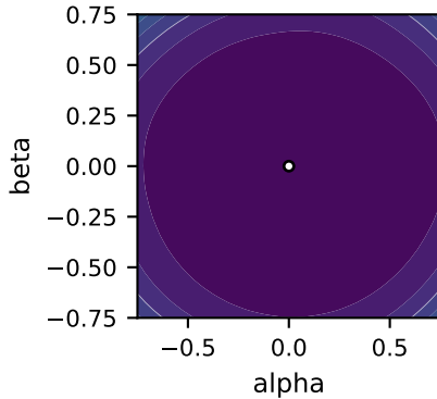
ASAM
