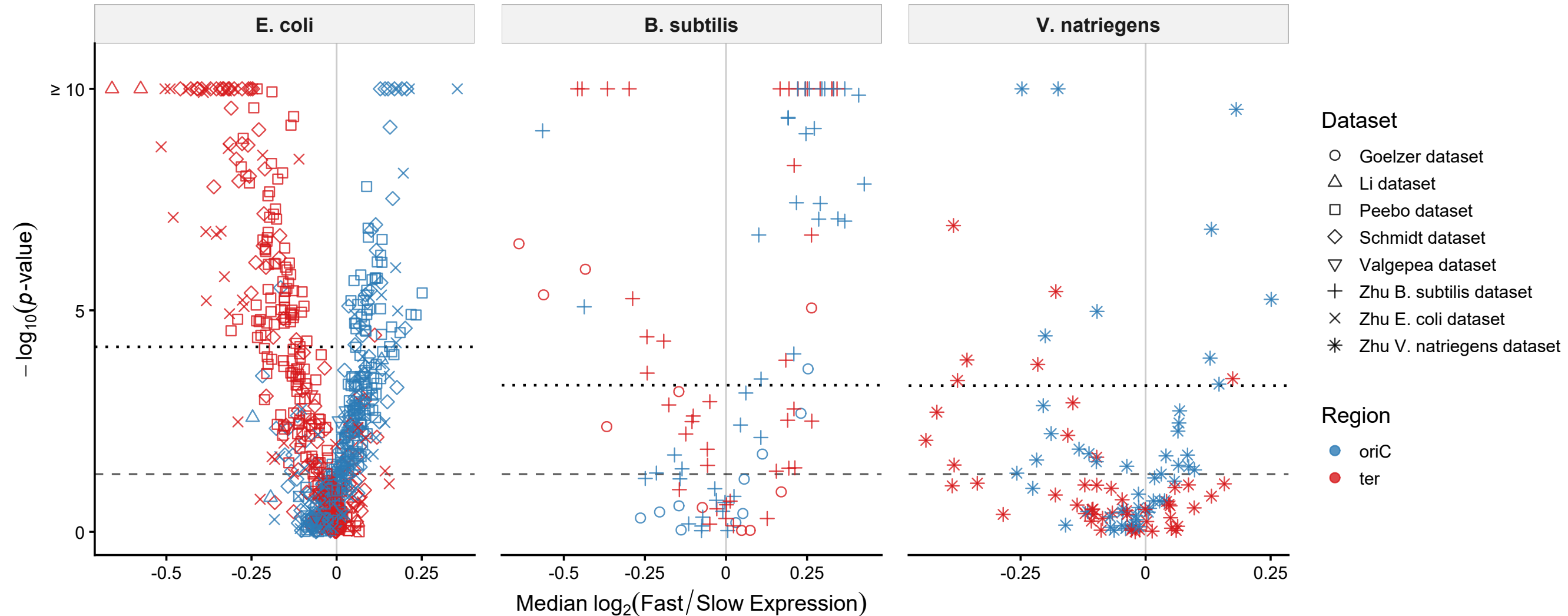
Meta-Volcano Plot proteomics_all_filtered_rel20_abs0.1
