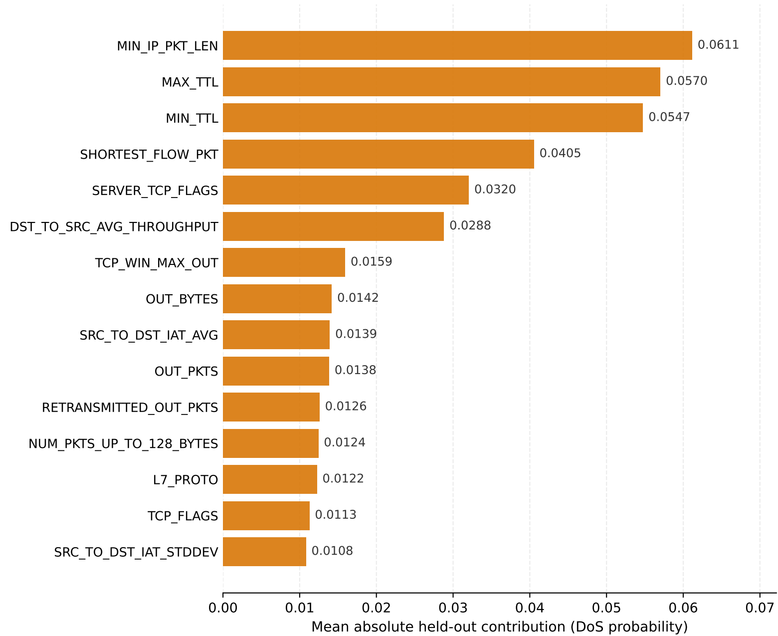
Random Forest
