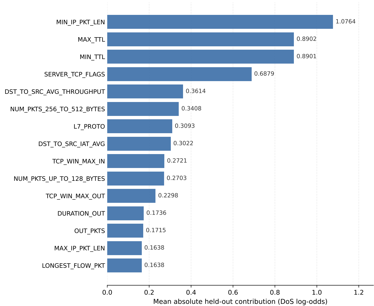
Logistic Regression
