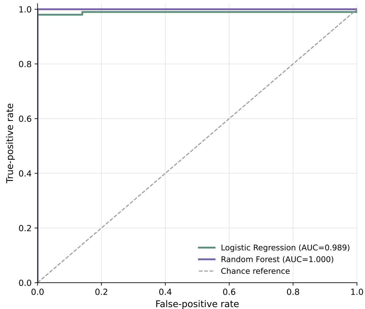
(a) Receiver operating characteristic
