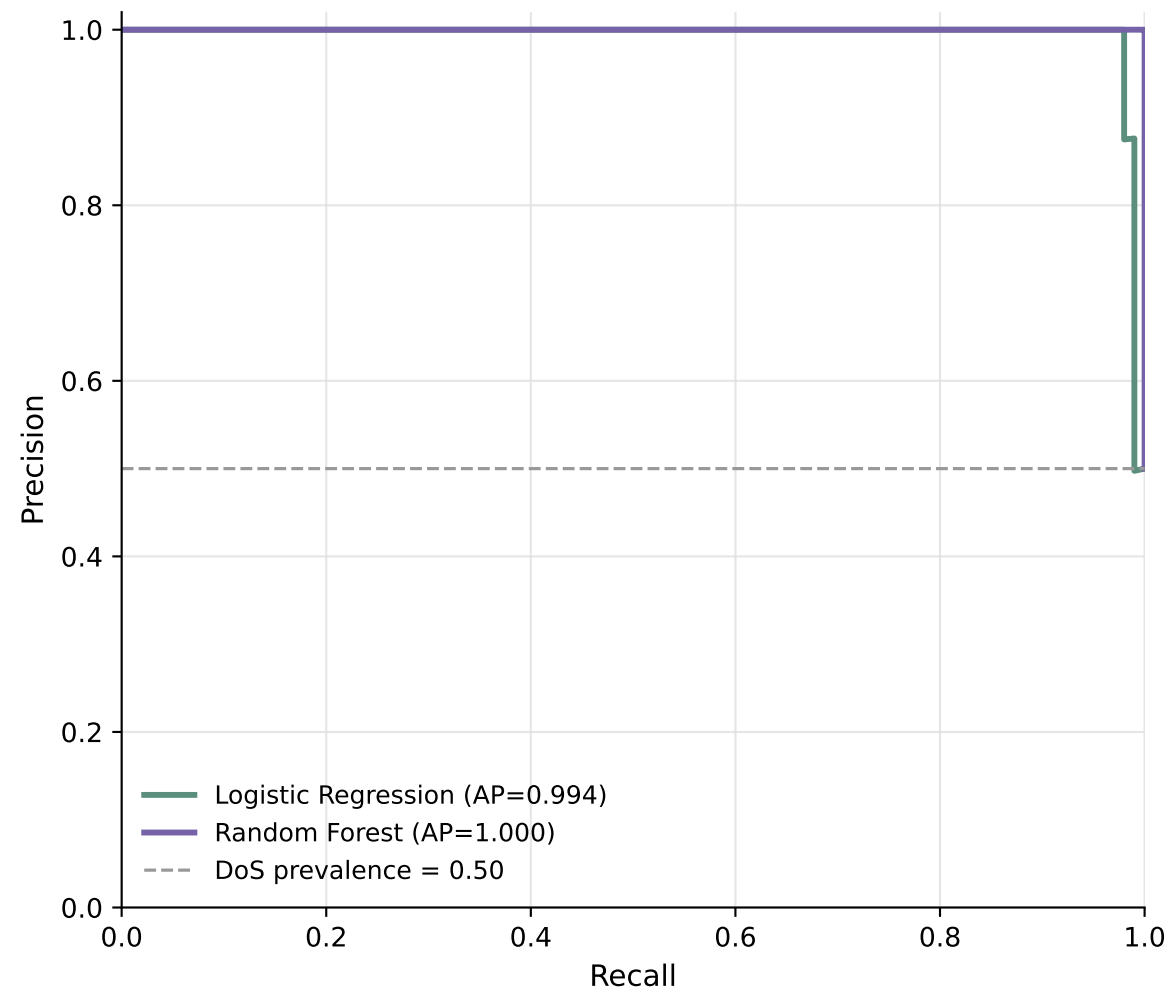
(b) Precision-recall curve
