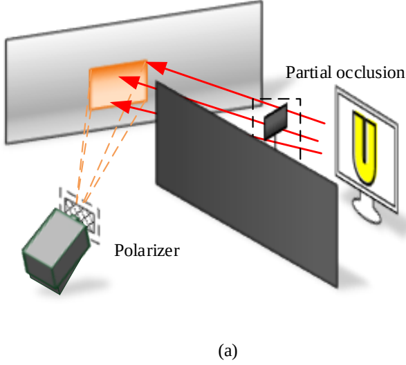
Fig. 5. Passive NLOS imaging: (a) Common constraints in passive NLOS imaging; (b) Passive NLOS imaging results.
