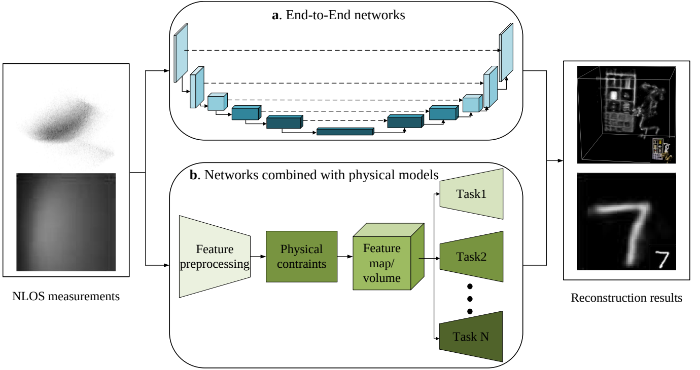
Fig. 6. Two types of models of NLOS imaging based on deep learning: (a) End-to-End Networks. (b) Physics-based Models. The reconstruction results in [18] and [135] are used as a demonstration.
