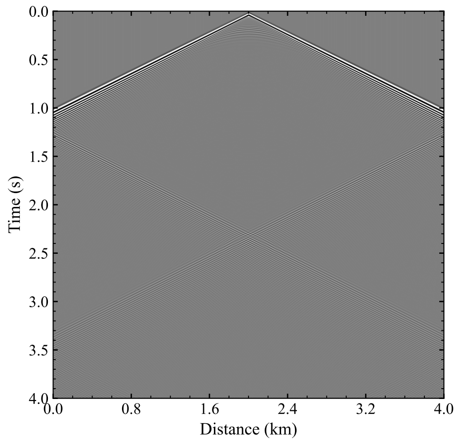
(b) CPML boundary
