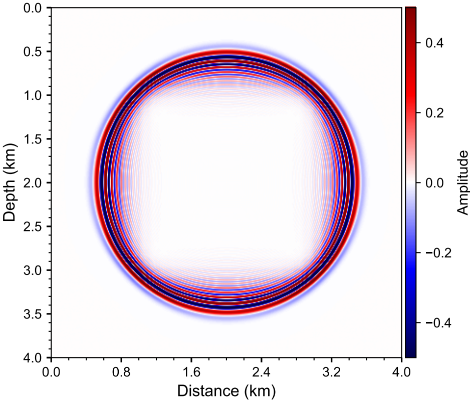
a. 2nd-order FD
