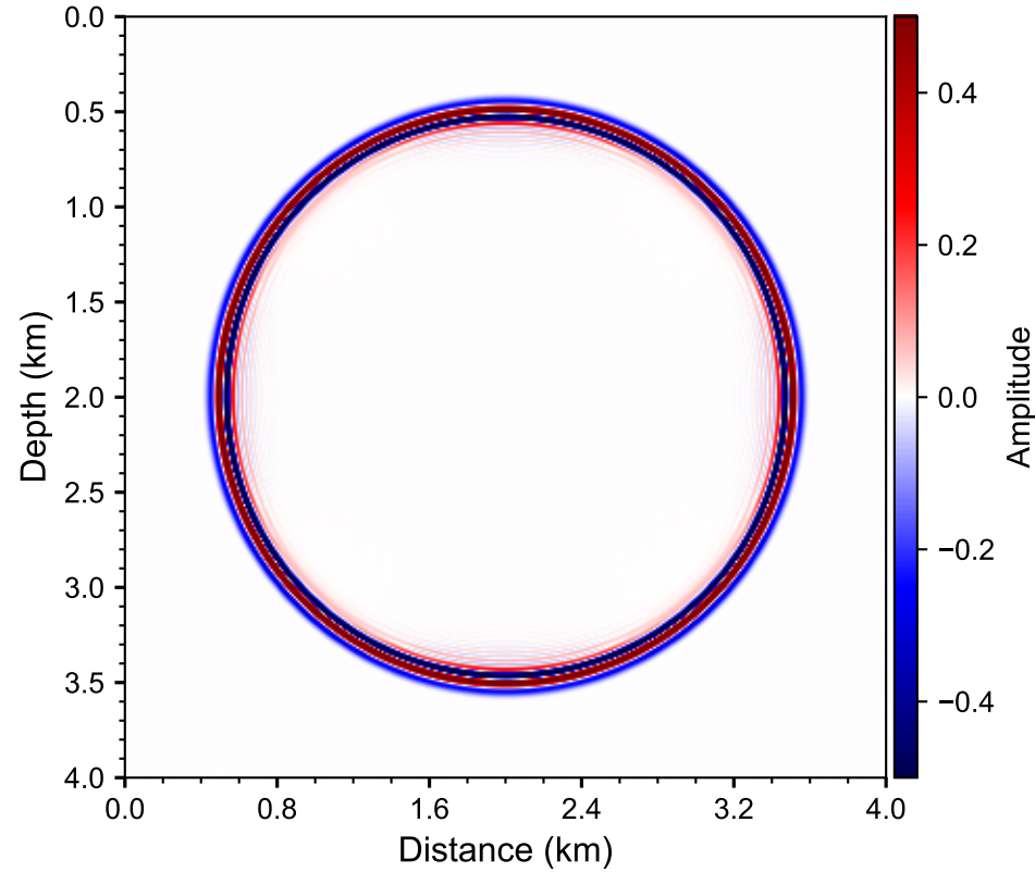
b. 4th-order FD
