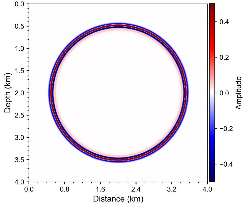
c. 6th-order FD
