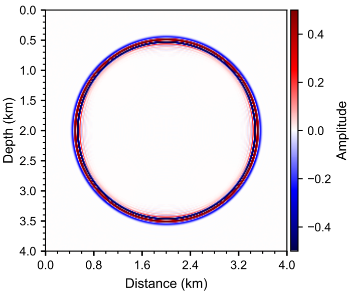
c. Grid spacing = 10 m
