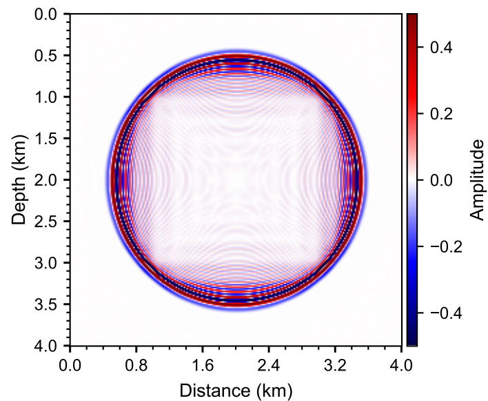
d. Grid spacing = 15 m
