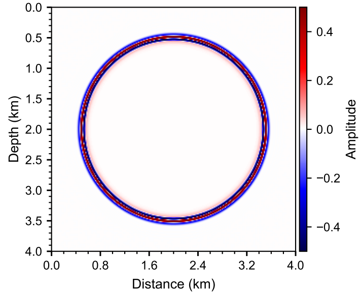
b. Grid spacing = 8 m
