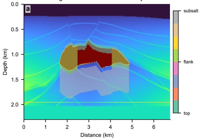
Target-zone illumination and RTM response
