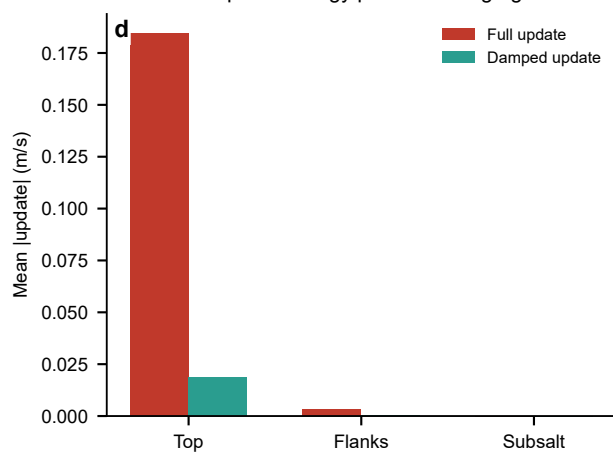
FWI update energy passed through gate
