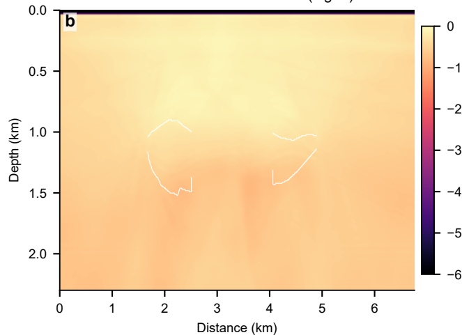
FWI update energy passed through gate
