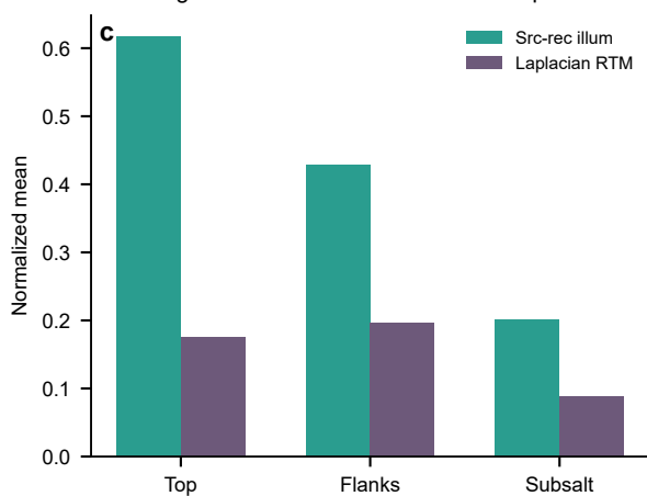
Target-zone illumination and RTM response
