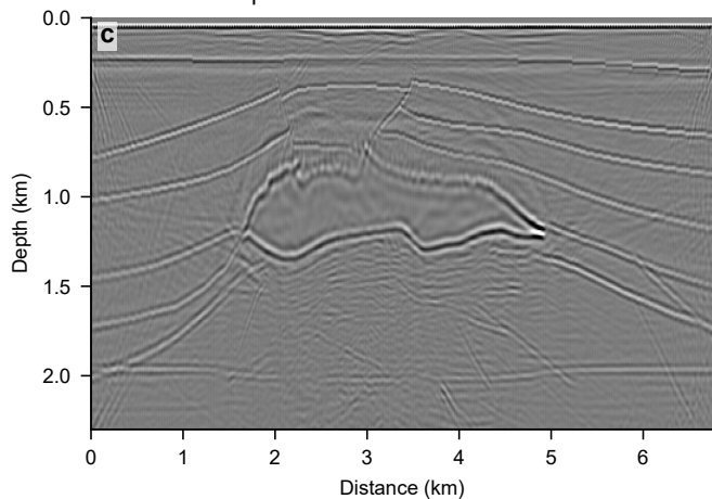
Laplacian source-normalized RTM
