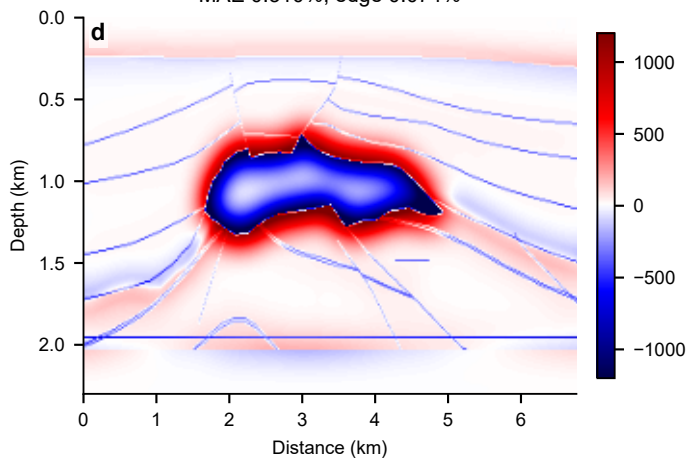
Spatial gate error MAE 0.310%, edge 0.074%
