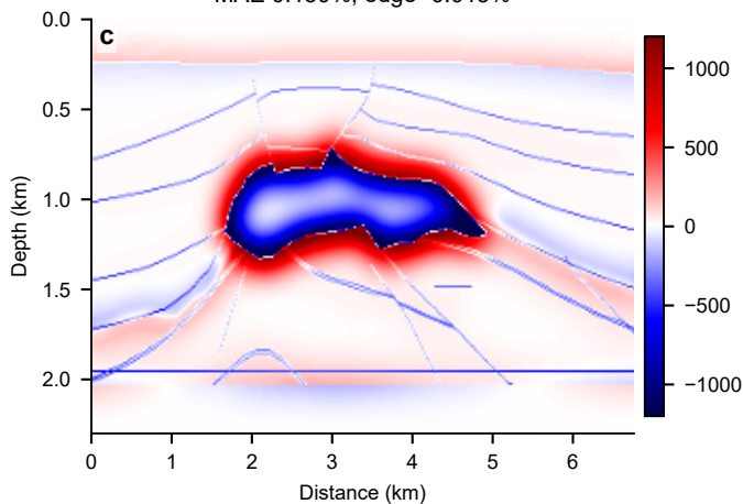
Global \alpha=0.1 error MAE 0.130%, edge -0.013%
