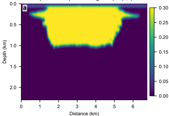
Global \alpha=0.1 error MAE 0.130%, edge -0.013%
