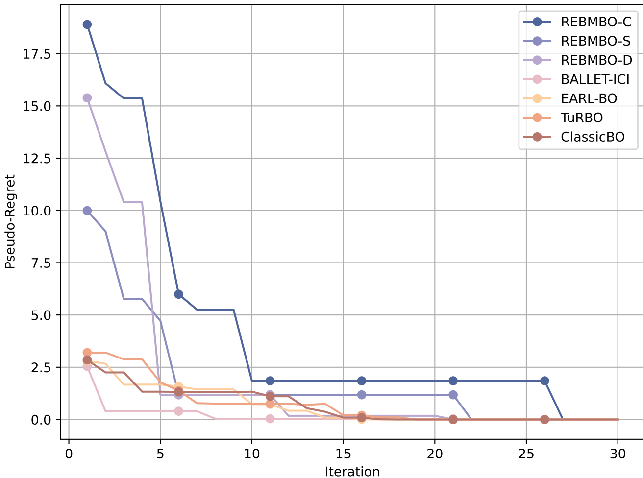
Ackley(5D)
