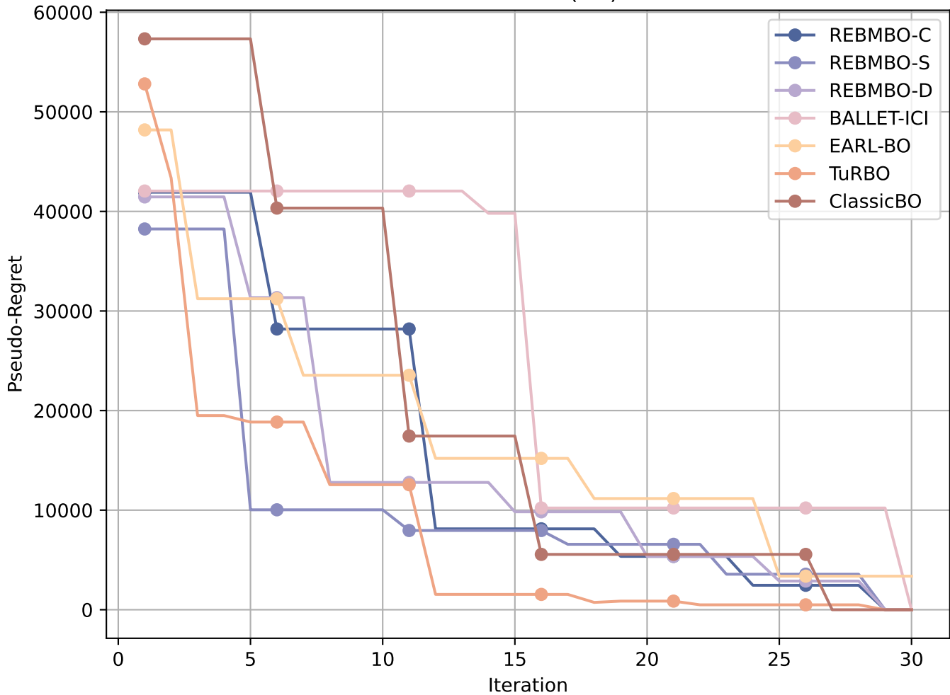
Rosenbrock(8D)
