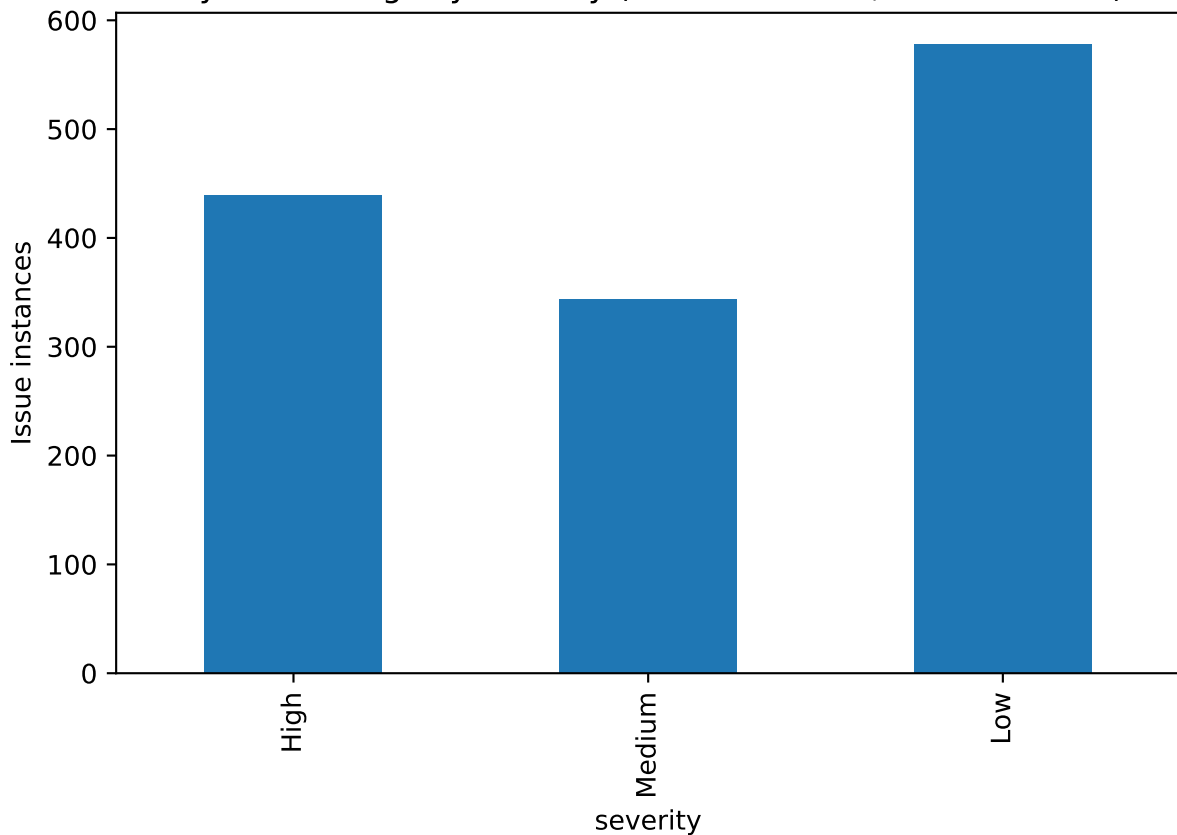
Mythril findings by severity (N=1361 issues, 487 contracts)
