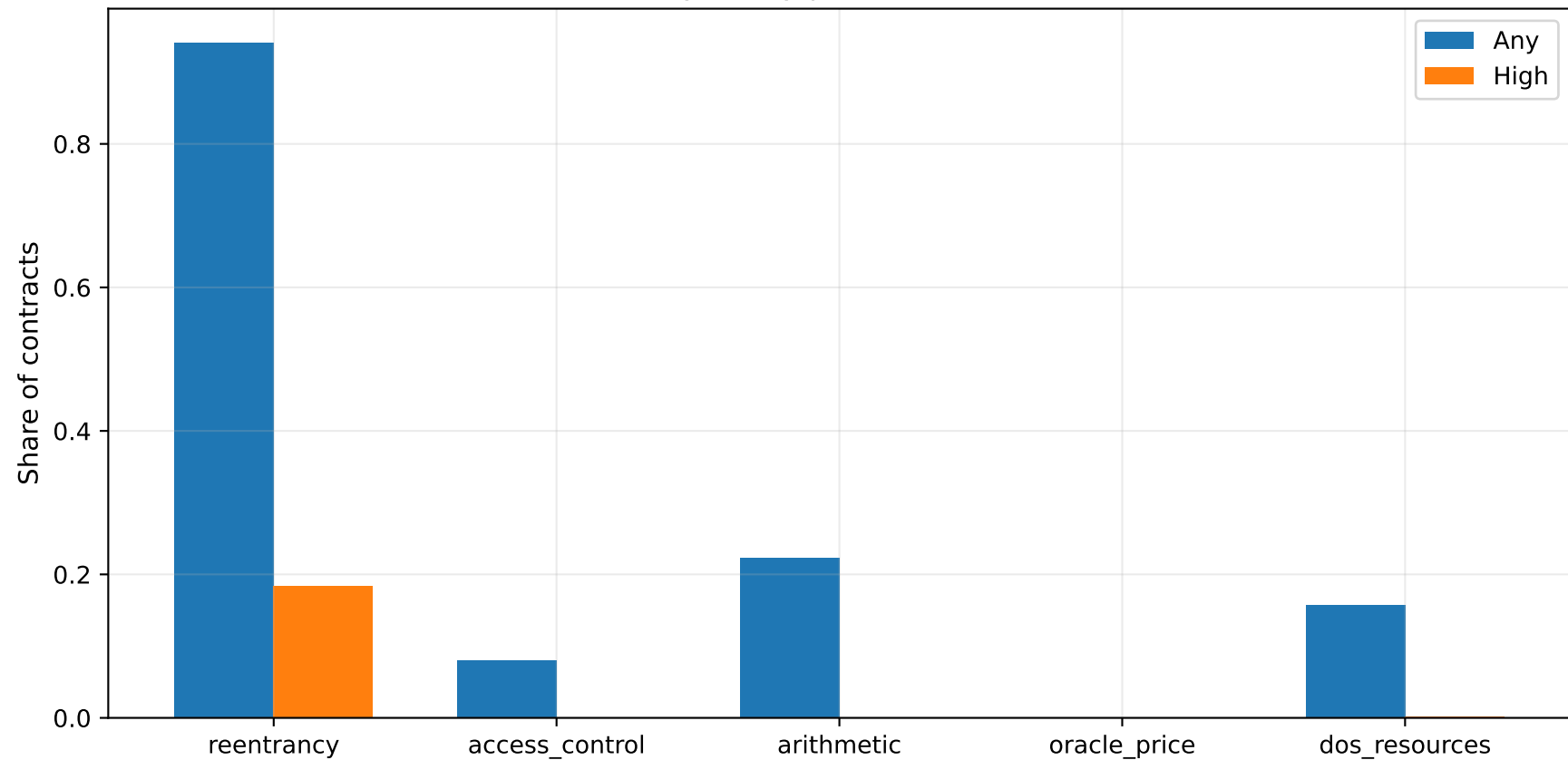
RQ1: Vulnerability-family prevalence (Slither contracts)
