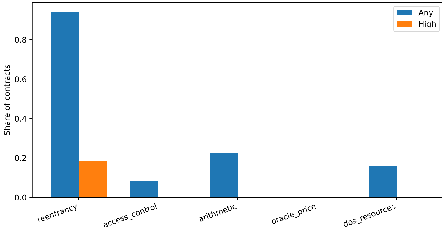
RQ1: Vulnerability-family prevalence (Slither contracts)
