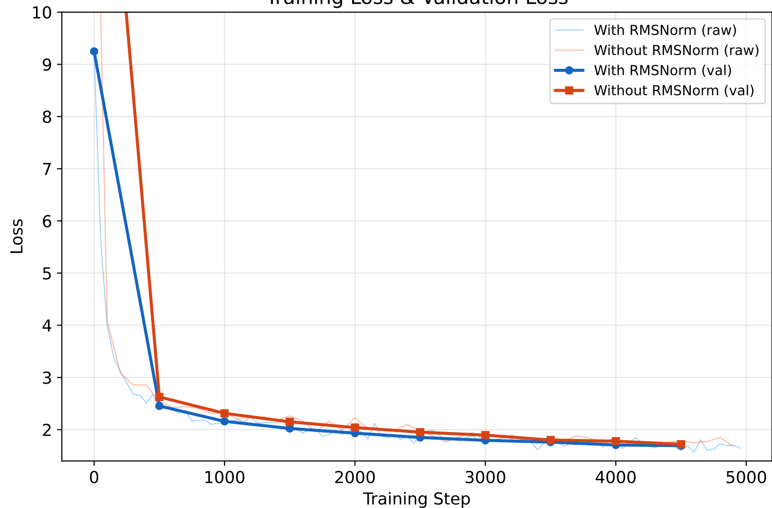
Training Loss & Validation Loss
