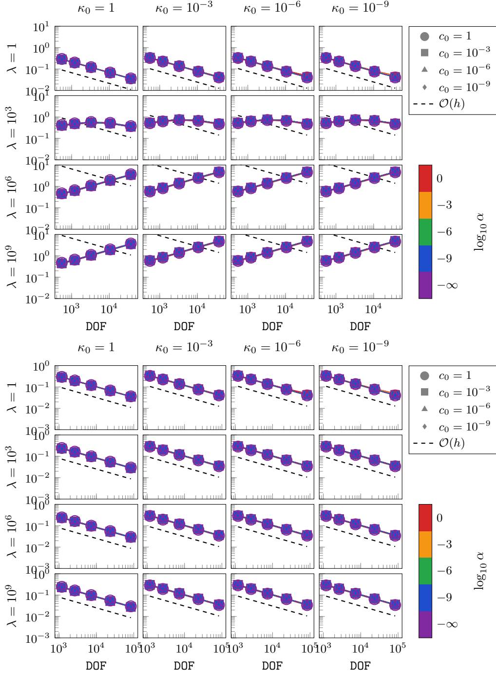
Figure 6.4: [Example 4, k = 0 ] Total weighted error ew versus number of degrees of freedom for \lambda \in \{1, 10^3, 10^6, 10^9\} (rows) and \kappa_0 \in \{1, 10^{-3}, 10^{-6}, 10^{-9}\} (columns), using the spaces (5.1)–(5.2) (top) and replacing \mathbb{H}_h^\xi by \tilde{\mathbb{H}}_h^\xi (bottom). In each panel, the colour indicates the value of \alpha \in \{0, 10^{-9}, 10^{-6}, 10^{-3}, 1\} (open markers and dashed lines for \alpha = 0 , which coincide with the curves for \alpha = 10^{-9} ) and the marker the value of c_0 \in \{1, 10^{-3}, 10^{-6}, 10^{-9}\} , and the black dashed line indicates the rate \mathcal{O}(h) .
