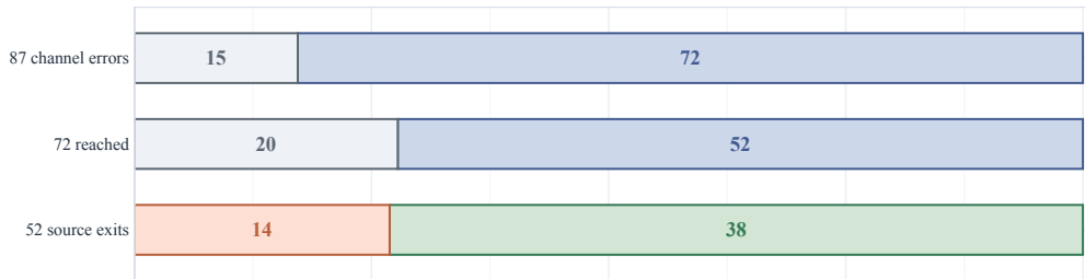
(b) The correct population the preservation bound that follows rests on 6 decisions
