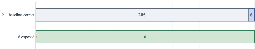
(b) The correct population the preservation bound that follows rests on 6 decisions
