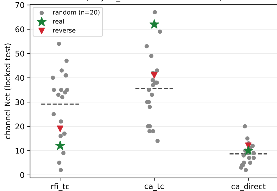
B. Mistral per-channel specificity (only ca_tc clears its random cloud)
