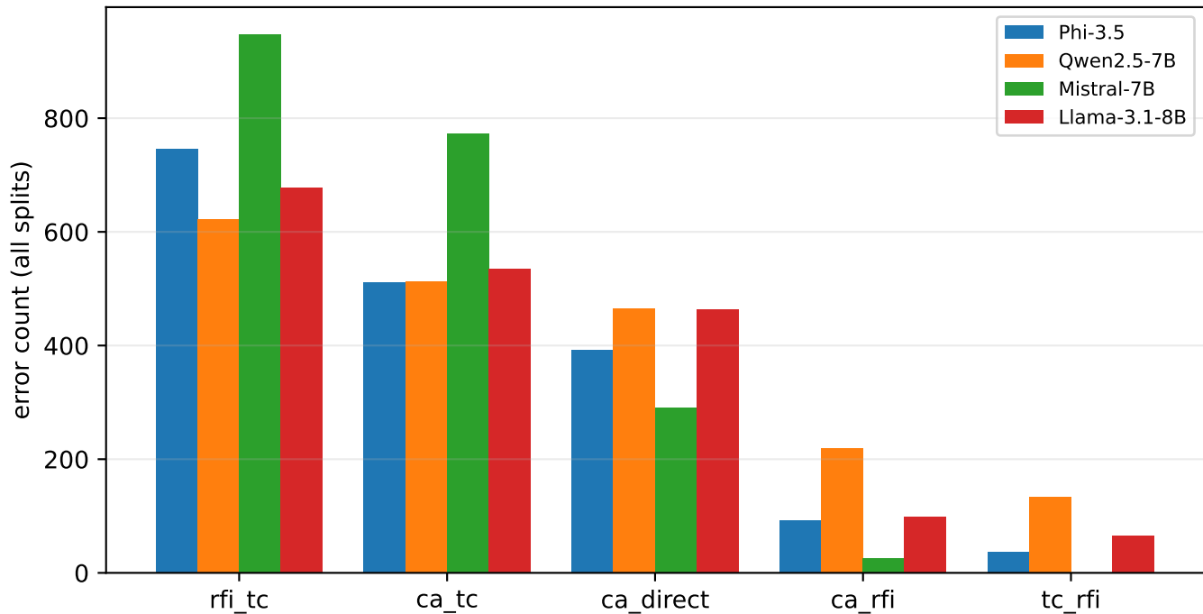
W2C error topology across four architectures (same dataset/split/readout)
