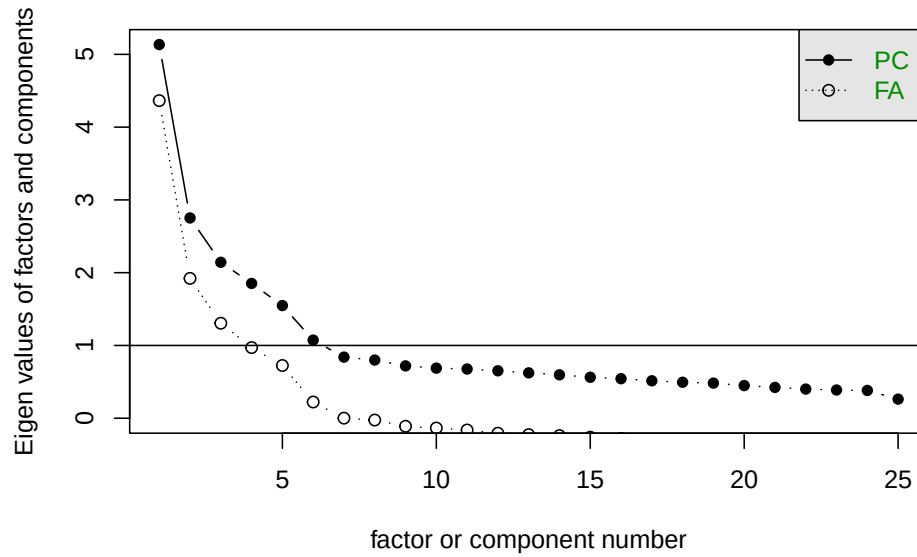
Scree plot
