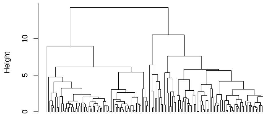
Cluster Dendrogram
