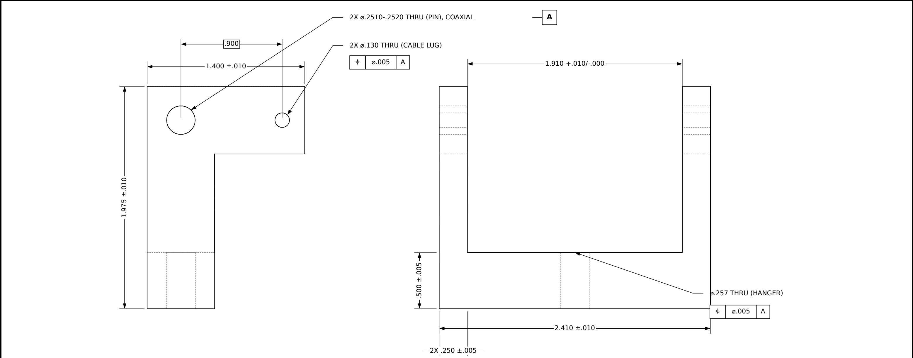
FRONT VIEW 2:1
