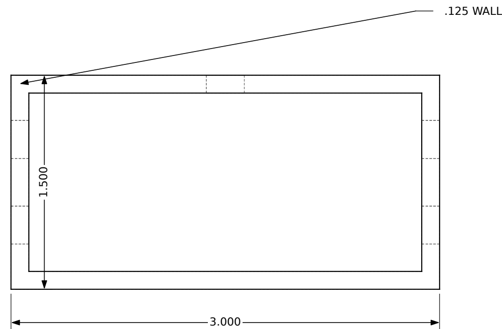
END VIEW 1.5:1
