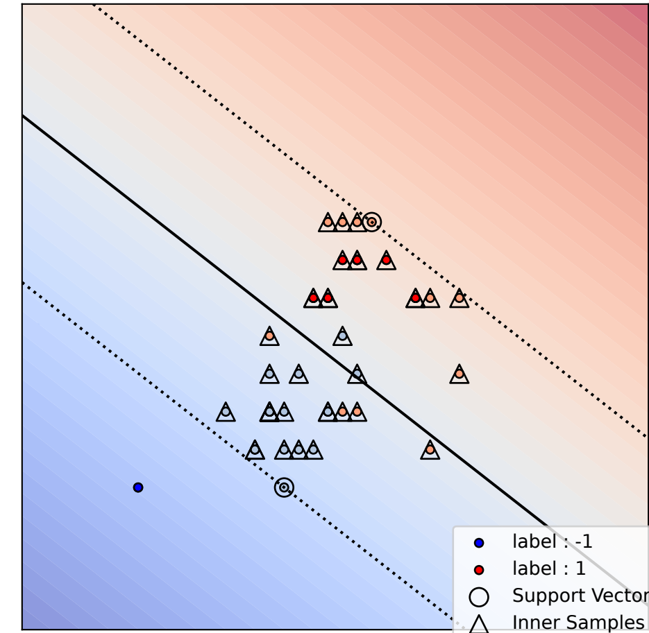
Agent 6
