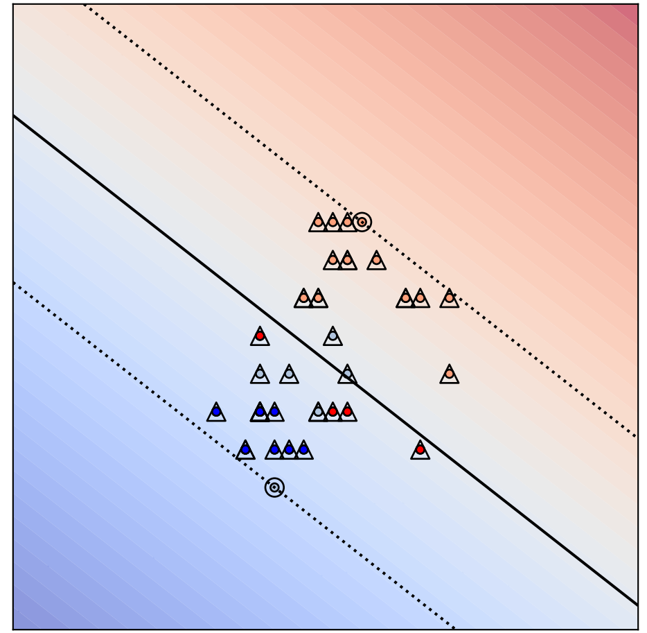
Agent 1
