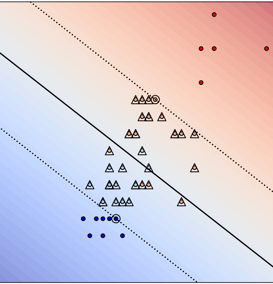
Agent 2
