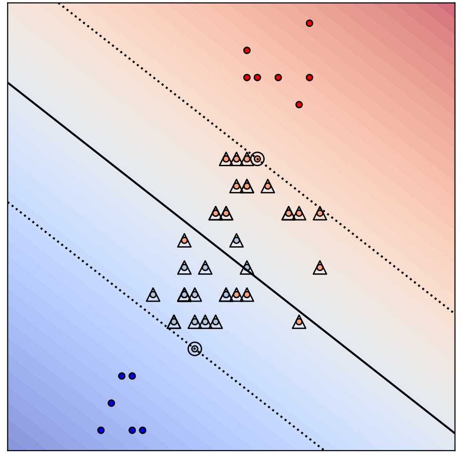
Agent 4
