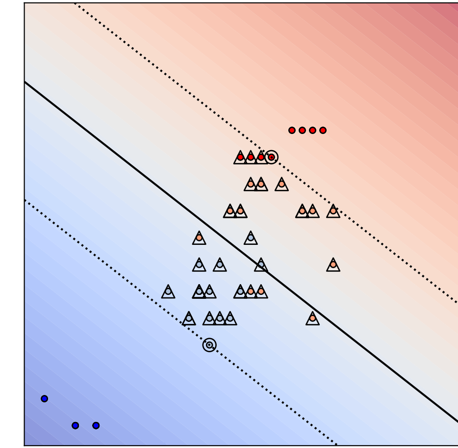
Agent 5
