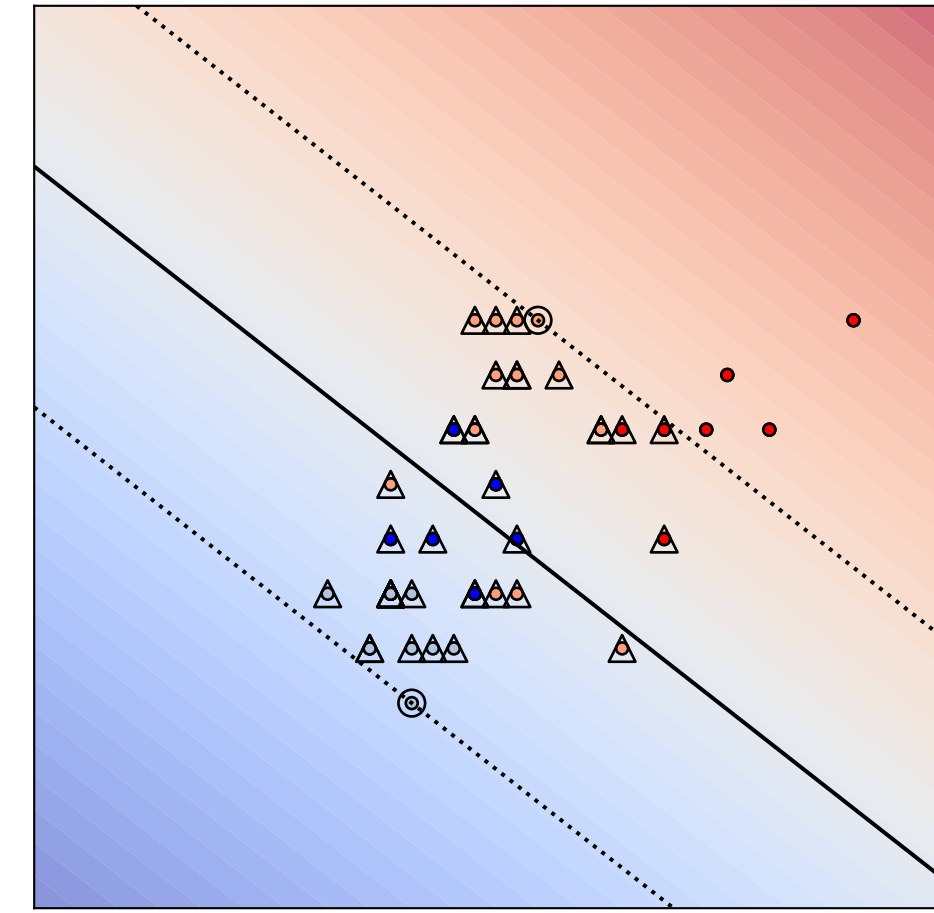
Agent 3
