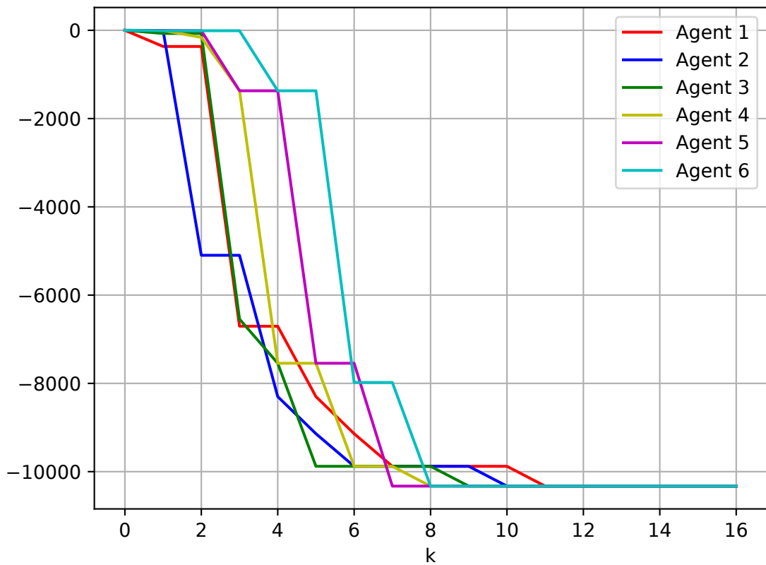
Objective value
