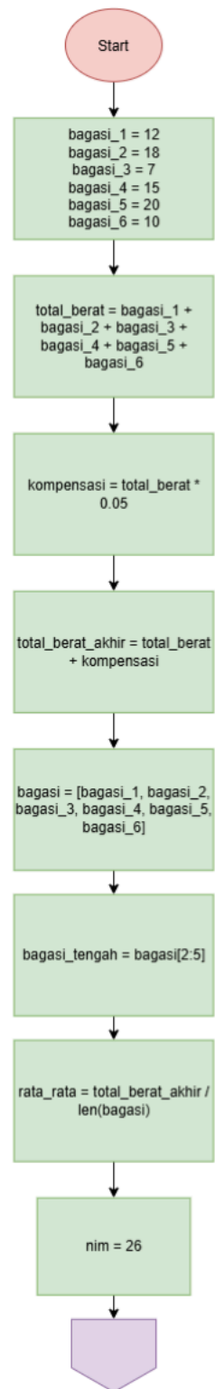
Gambar 1.1 Flowchart
