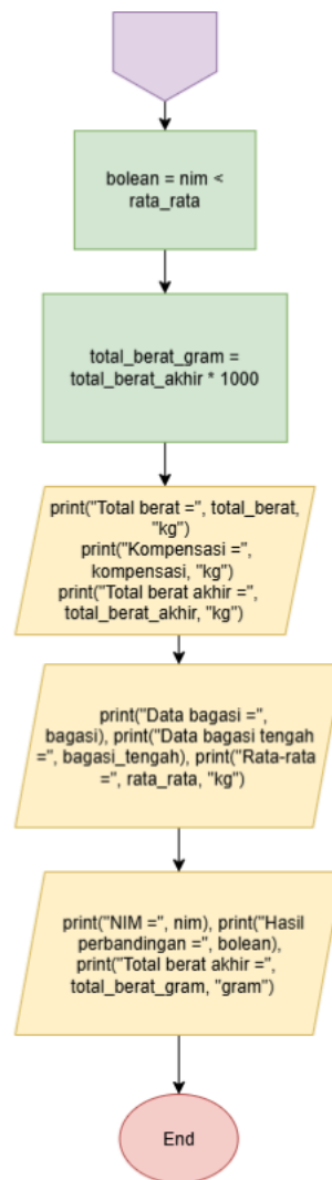
Gambar 1.2 Flowchart
