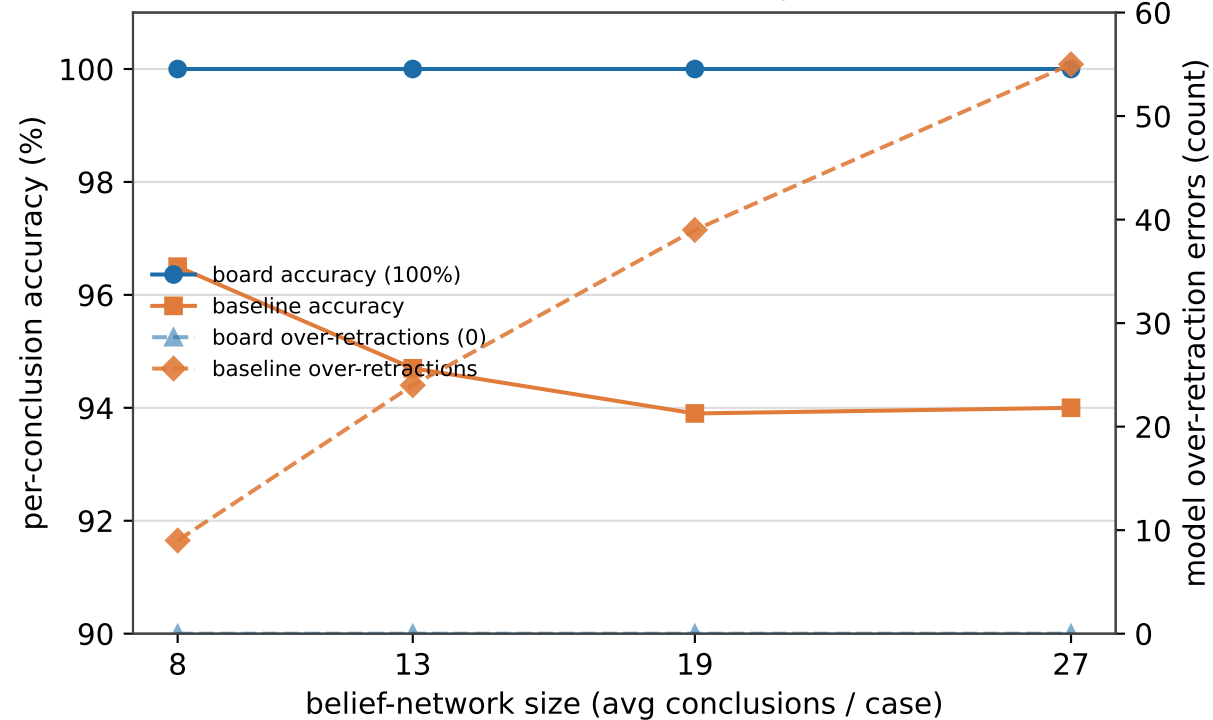
Belief revision: board exact + scale-invariant; model erodes with scale
