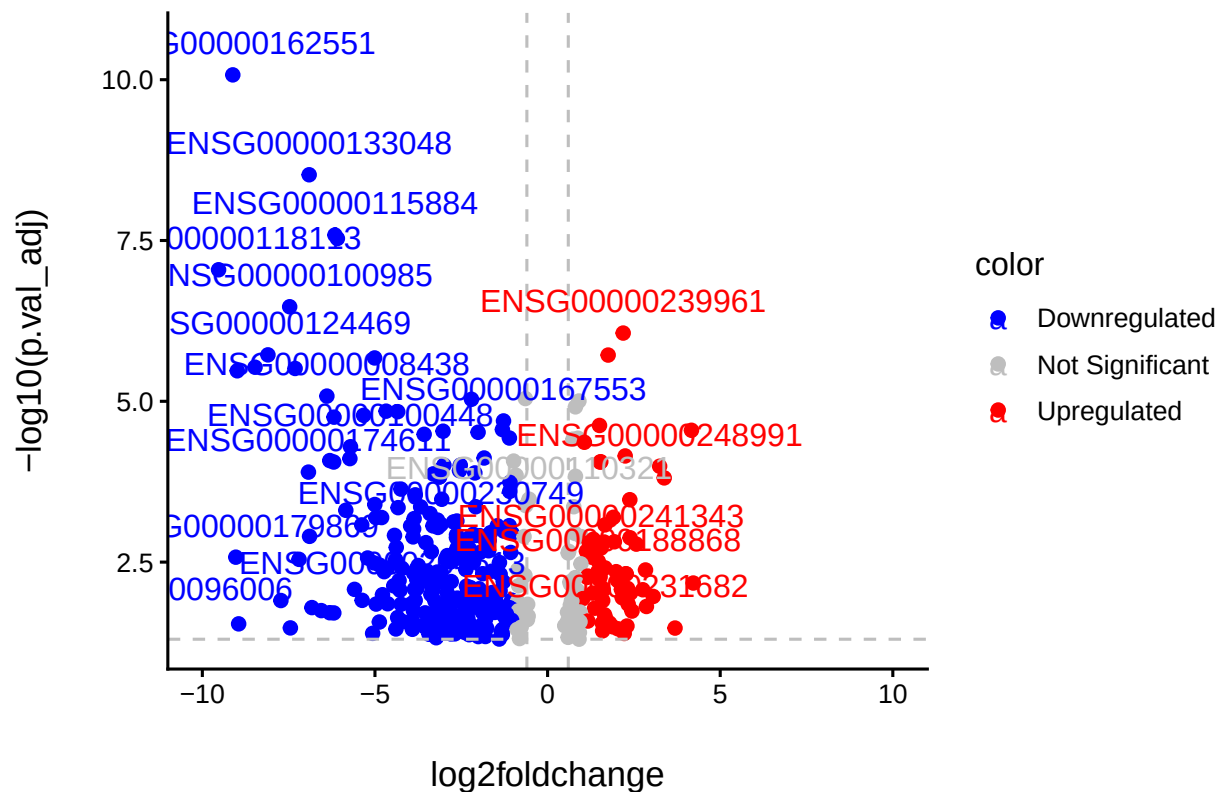
Volcano Plot: healthy-covid19
