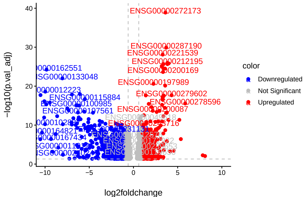
Volcano Plot: convalescent-covid19
