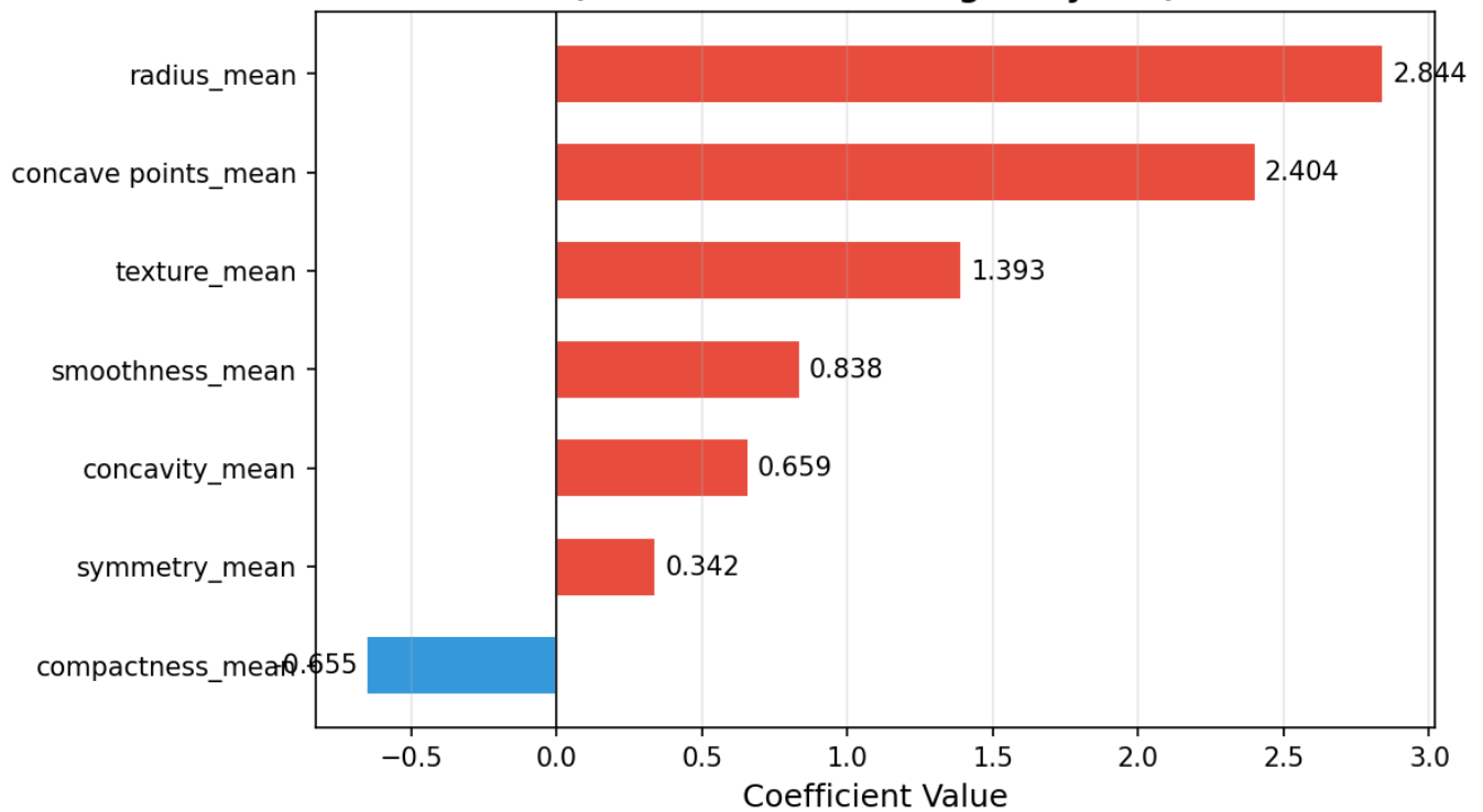
Logistic Regression — Feature Coefficients (Red = increases malignancy risk)
