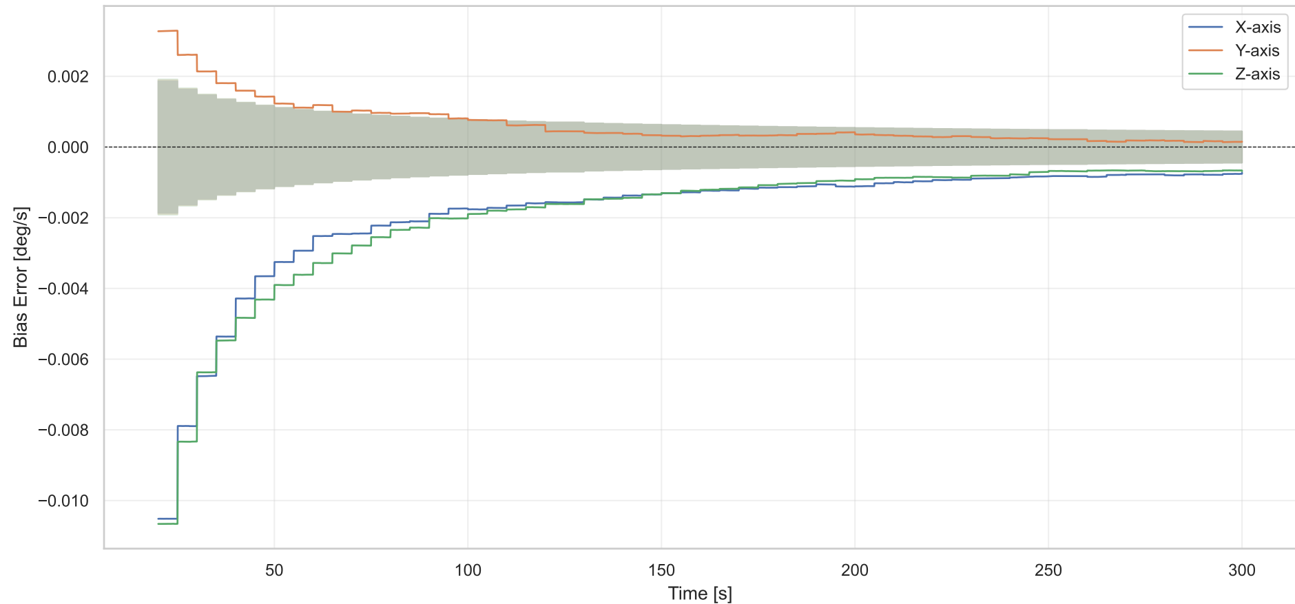
Gyro Bias Estimation Error - Steady State (with \pm 3\sigma bounds)
