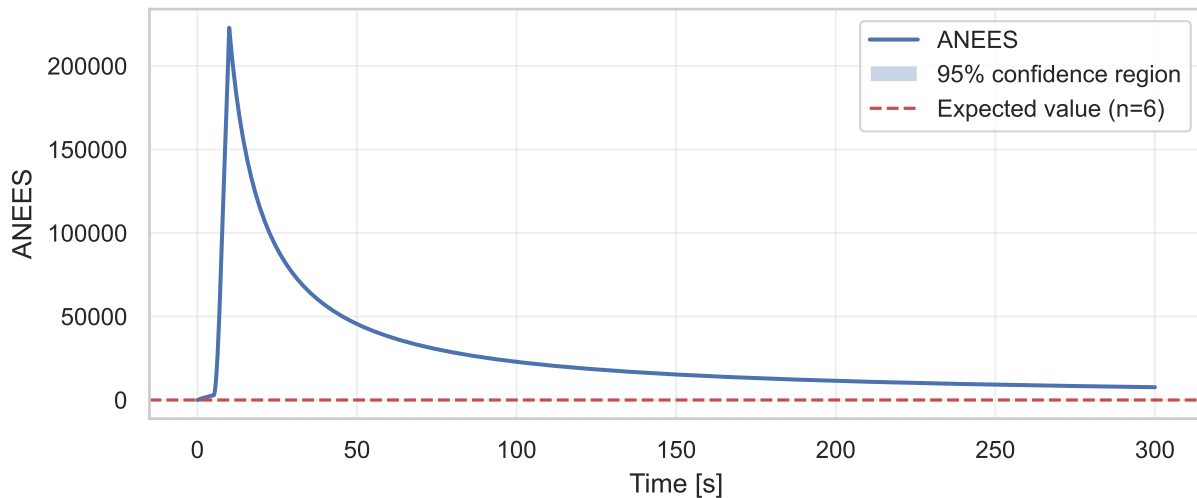
Average NEES with \chi^2 Confidence Bounds
