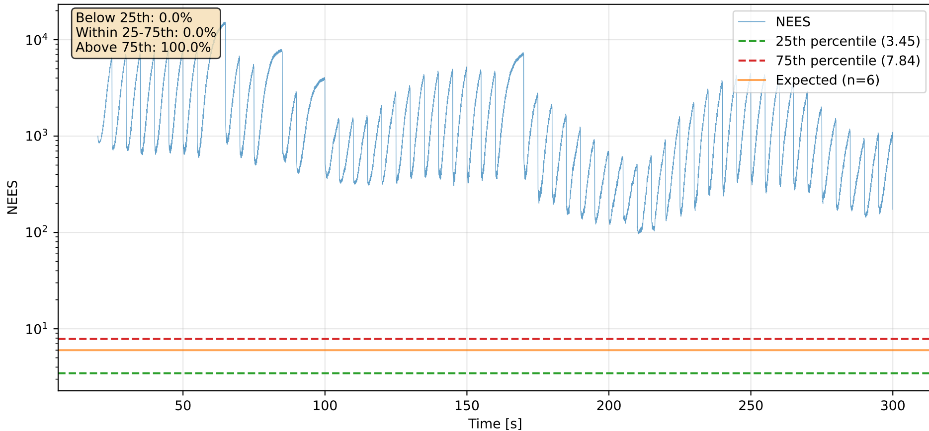
Normalized Estimation Error Squared (NEES) - Steady State
