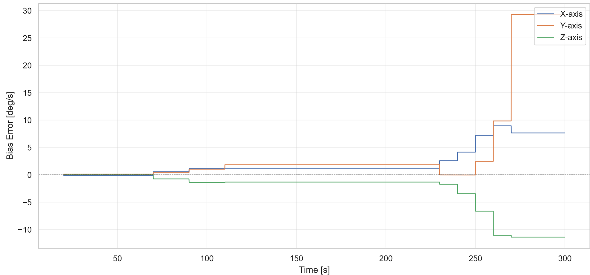
FGO Gyro Bias Estimation Error - Steady State
